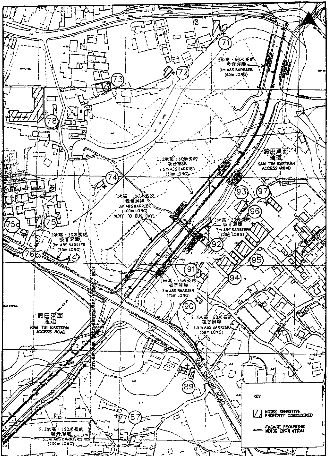
Figure 2 - Direct Road Traffic Noise Mitigation Measures for Kam Tin Eastern Access Road (North & East Section)
