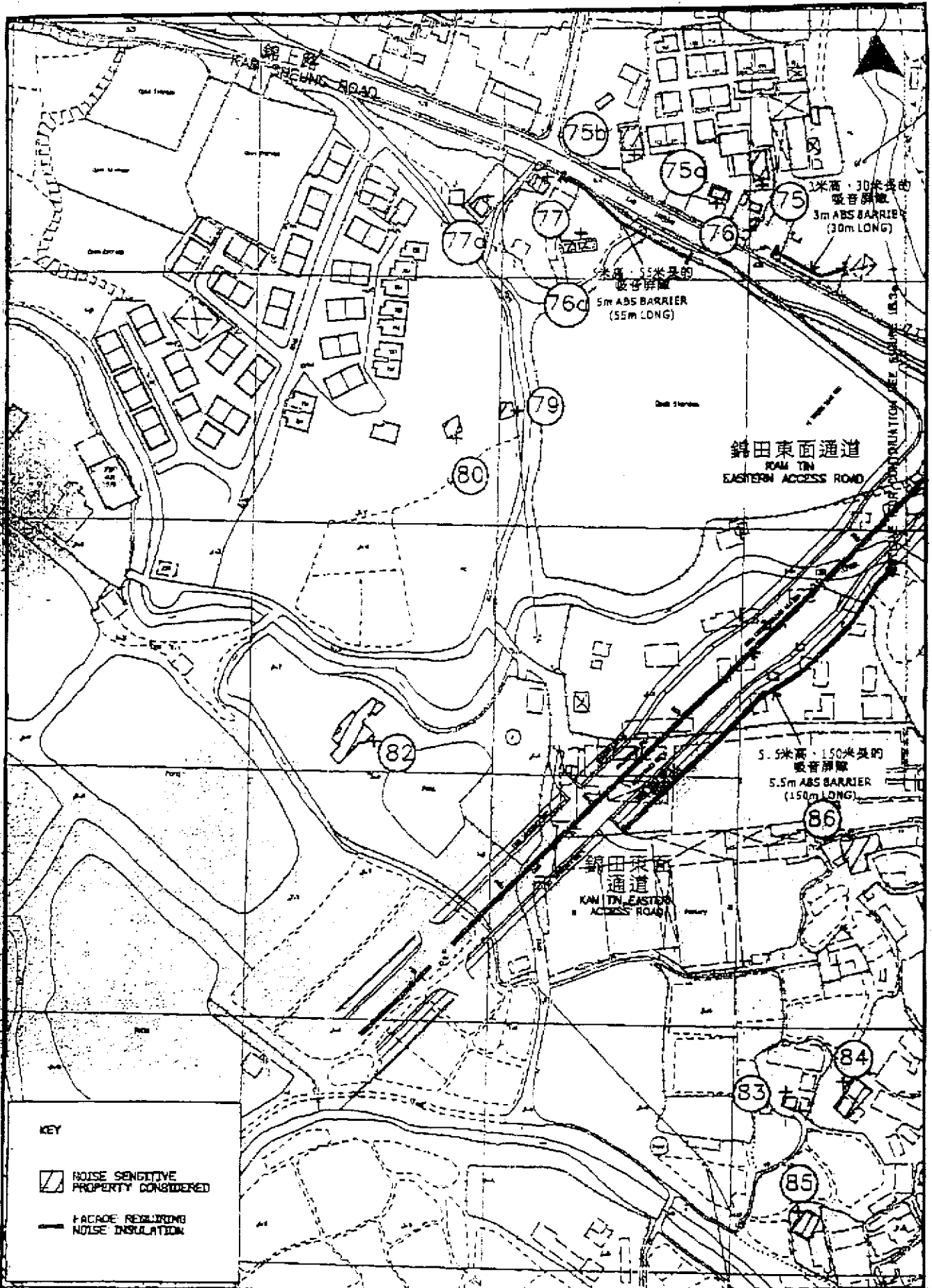
Figure 3 - Direct Road Traffic Noise Mitigation Measures for Kam Tin Eastern Access Road (South & West Section)
