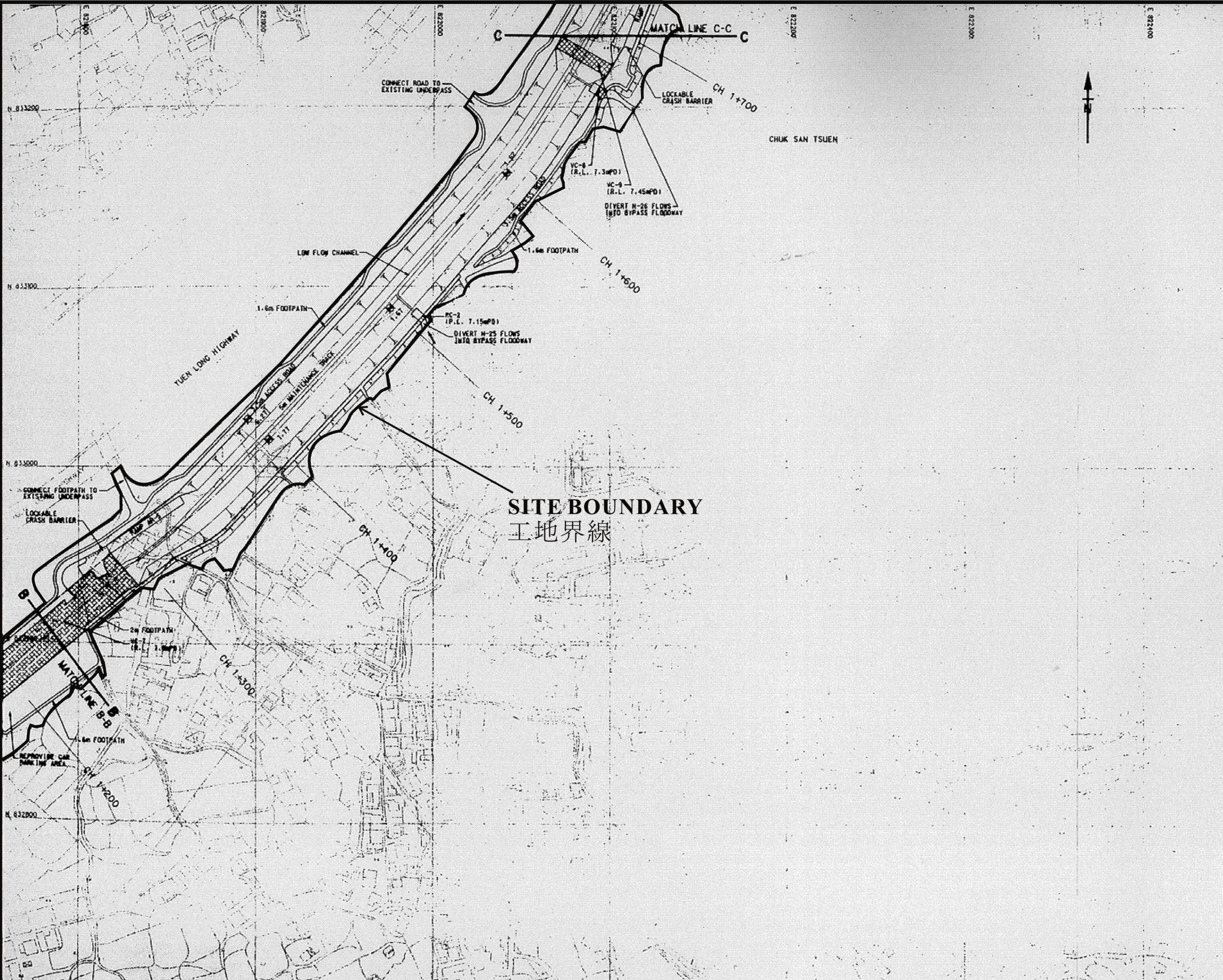
Figure 1.3 Location Plan of Yuen Long Bypass Floodway
