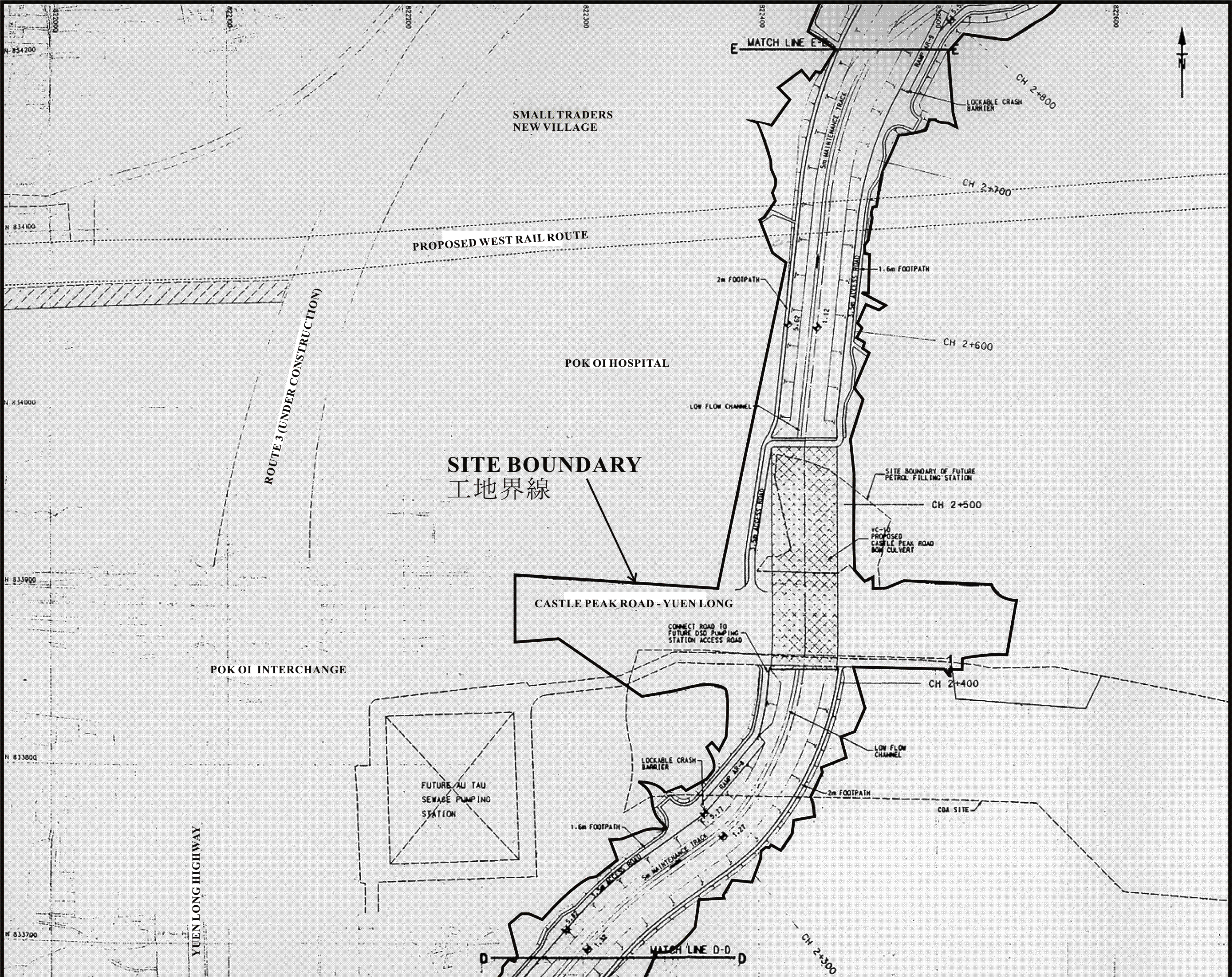
Figure 1.5 Location Plan of Yuen Long Bypass Floodway
