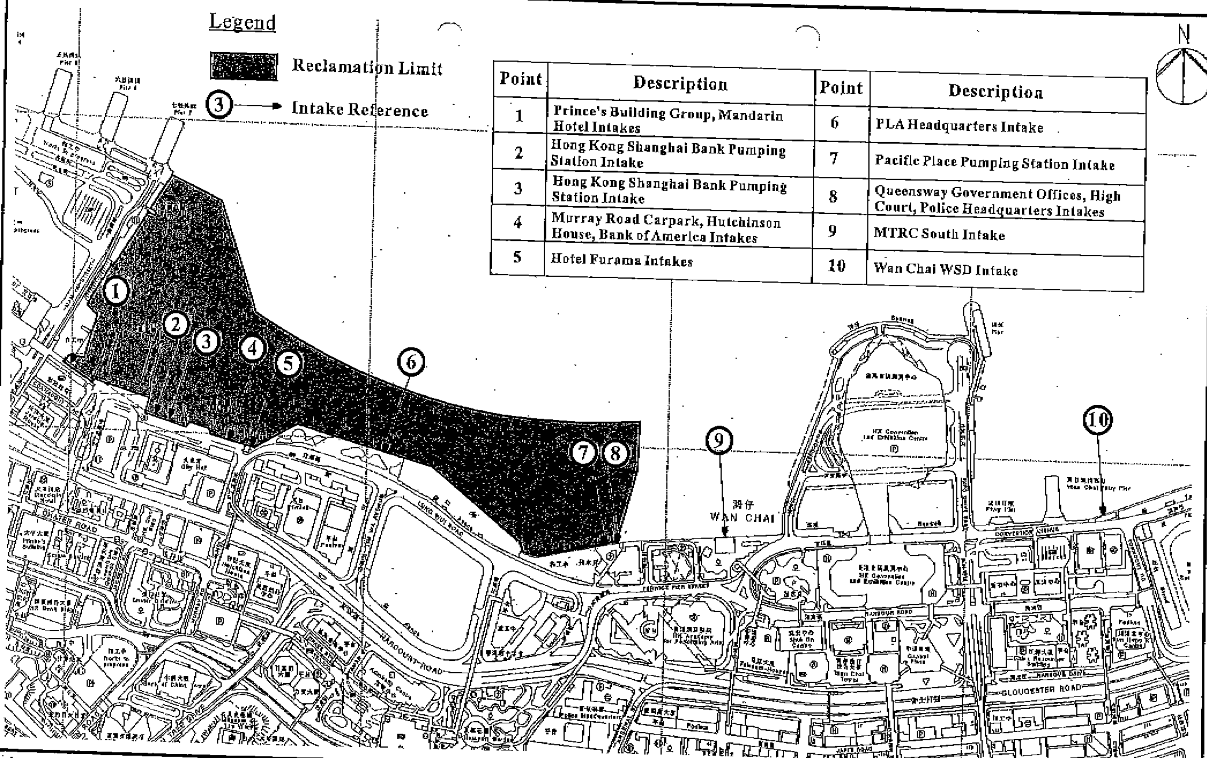
中環填海計劃第III期 Central Reclamation Phase III 環境許可証編號 FEP-01/122/2003 Environmental Permit Number FEP-01/122/2003 Figure 6 : Locations of Cooling Water Intakes & Wan Chai WSD Intake
