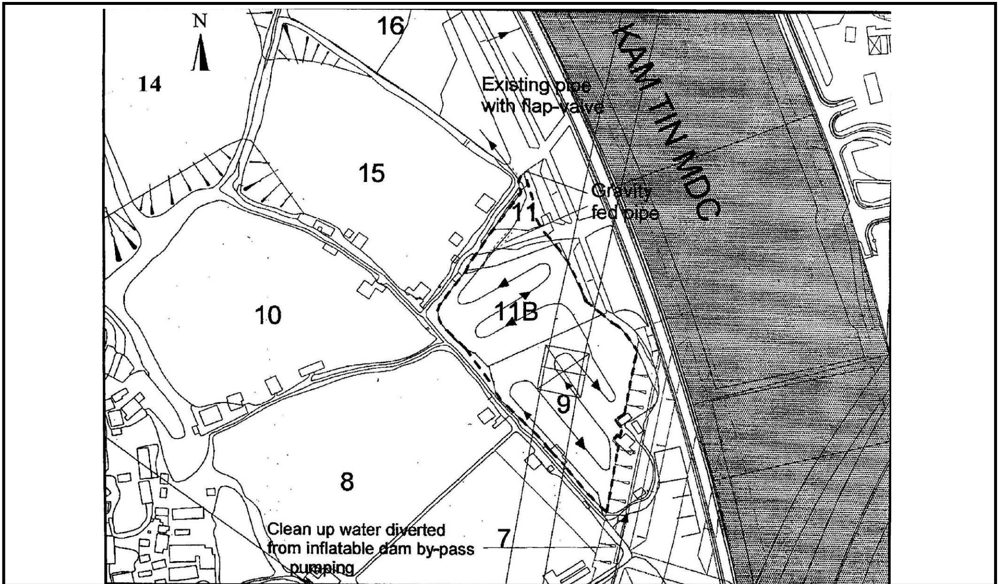
Location Plan of Ponds 9, 11 and 11B
