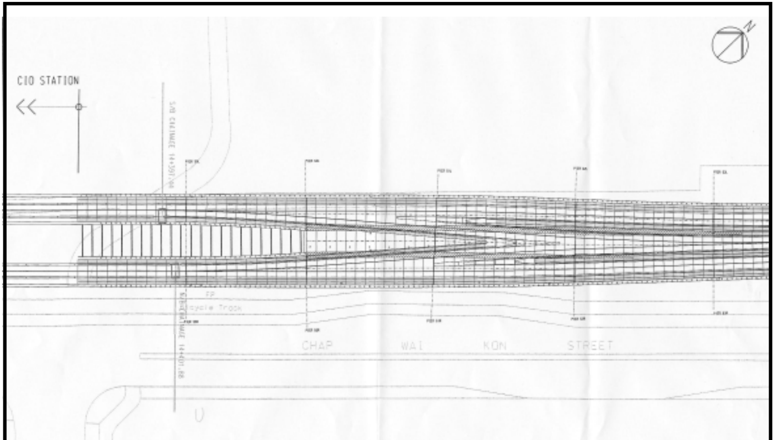
Figure 11 Point machine locations between City One Station and Shek Mun Station (Extracted from the Application VEP-085/2003)
