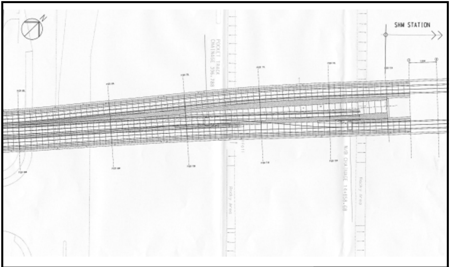
Figure 13 Point machine locations between City One Station and Shek Mun Station (Extracted from the Application VEP-085/2003)
