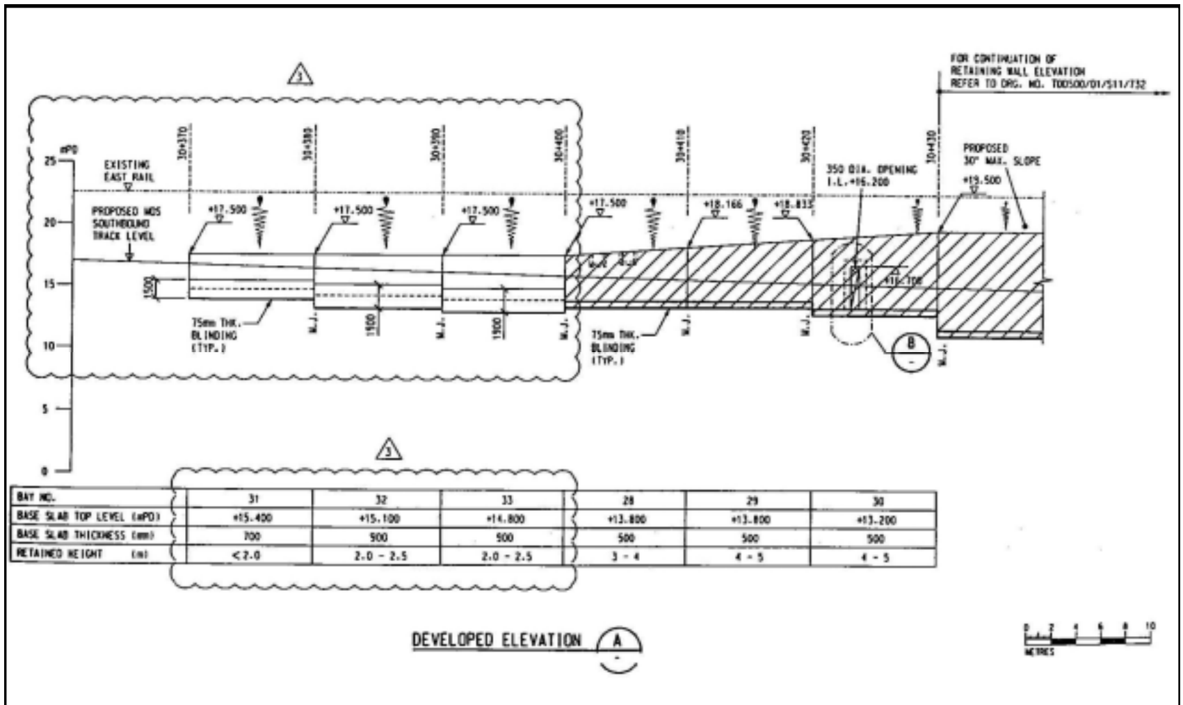
Figure 18 Retaining Wall RW3A (Extracted from the Application VEP-157/2004)
