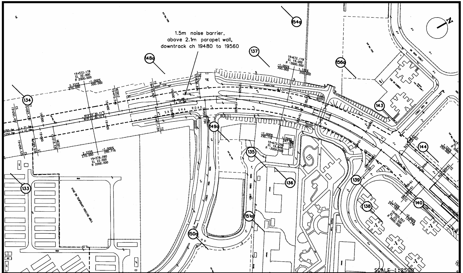
Figure 9 Noise Barriers and Enclosures (Extracted from Technical Annex F1 of the EIA Report)
