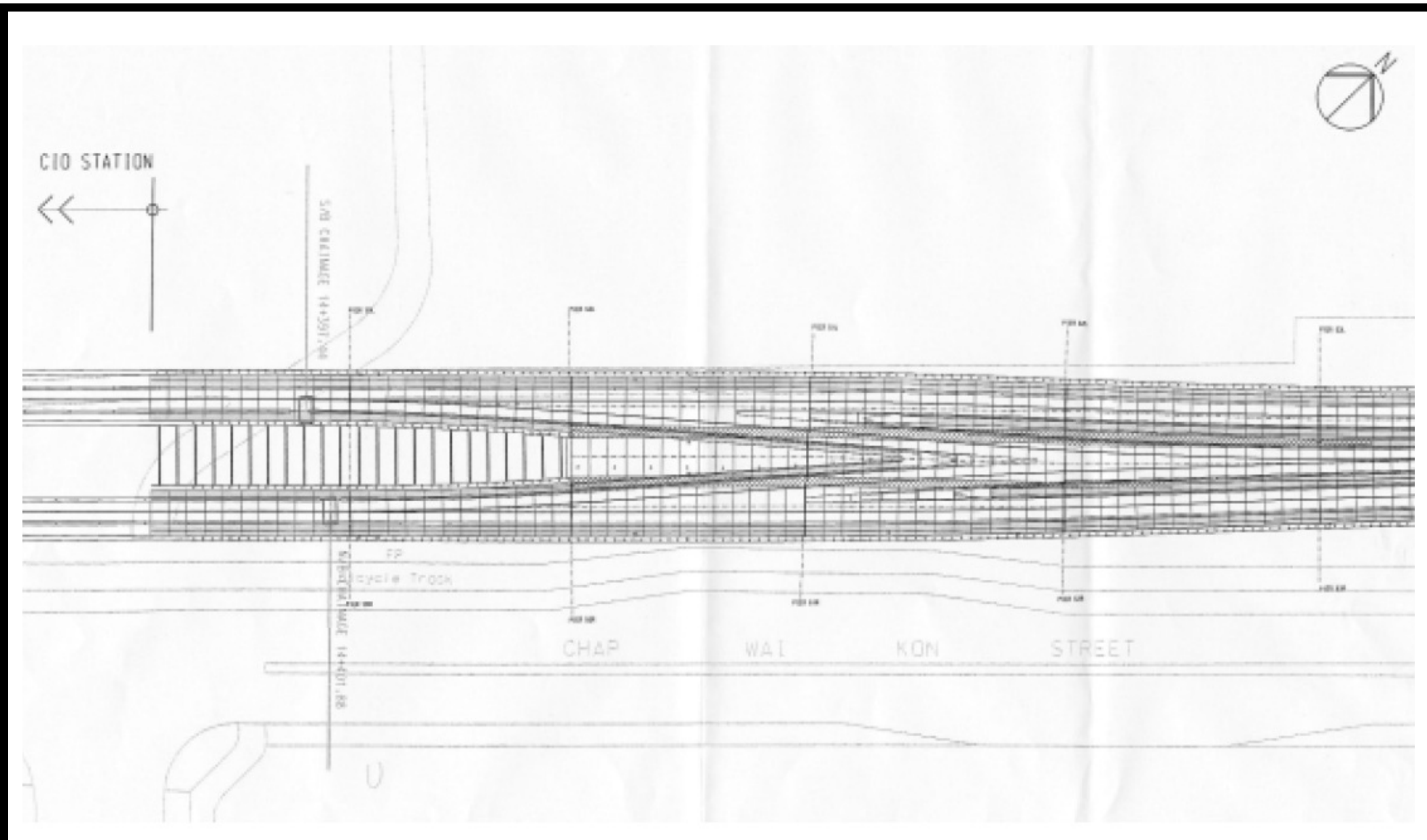
Project Title: East Rail Extensions - Tai Wai to Ma On Shan Figure 11: Point machine locations between City One Station and Shek Mun Station [Extracted from the Figure 11 of FEP Application (Application No.: FEP-132/2012)]
