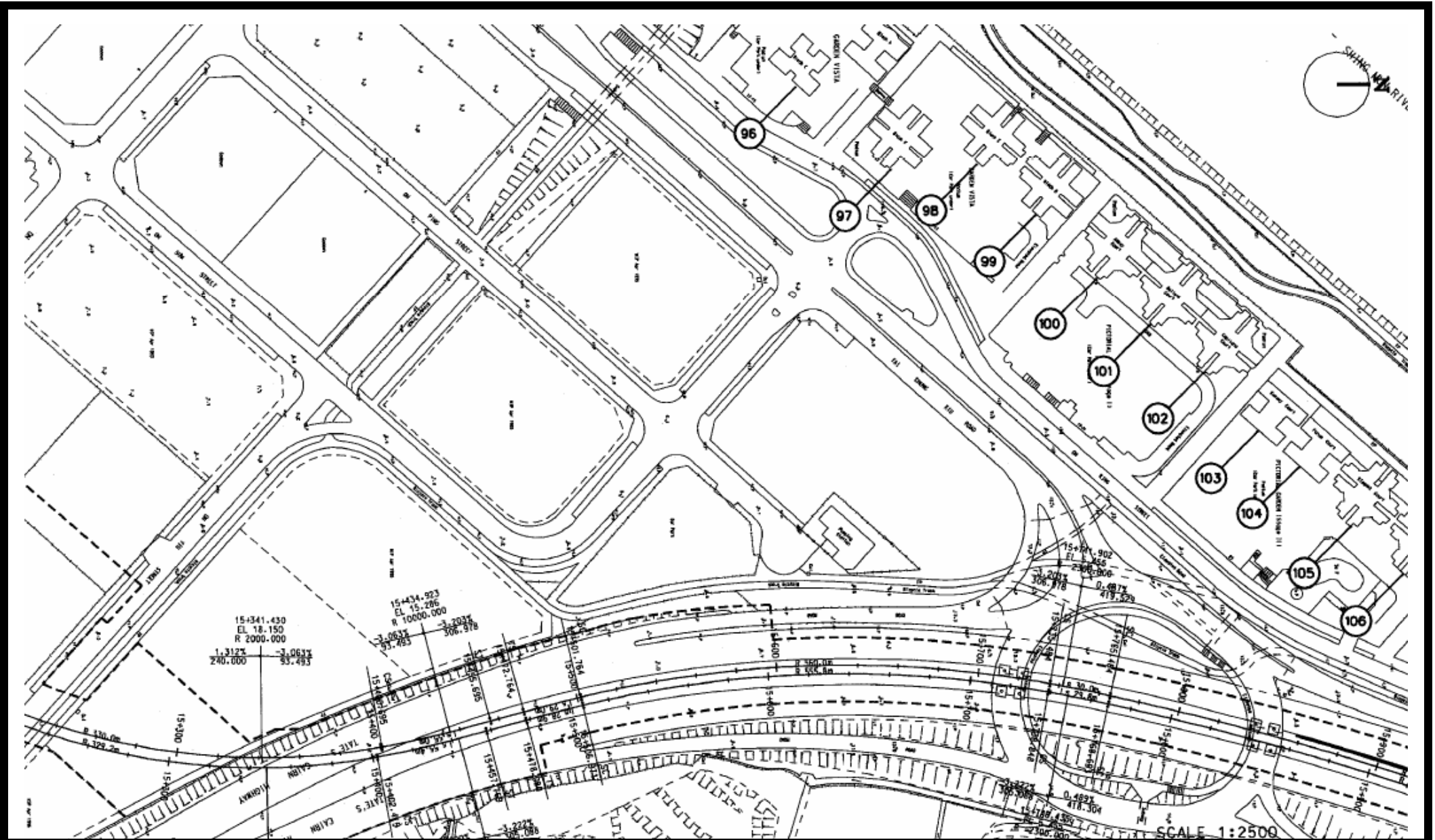
Project Title: East Rail Extensions - Tai Wai to Ma On Shan Figure 5: Noise Barriers and Enclosures [Extracted from the Figure 5 of FEP Application (Application No.: FEP-132/2012)]
