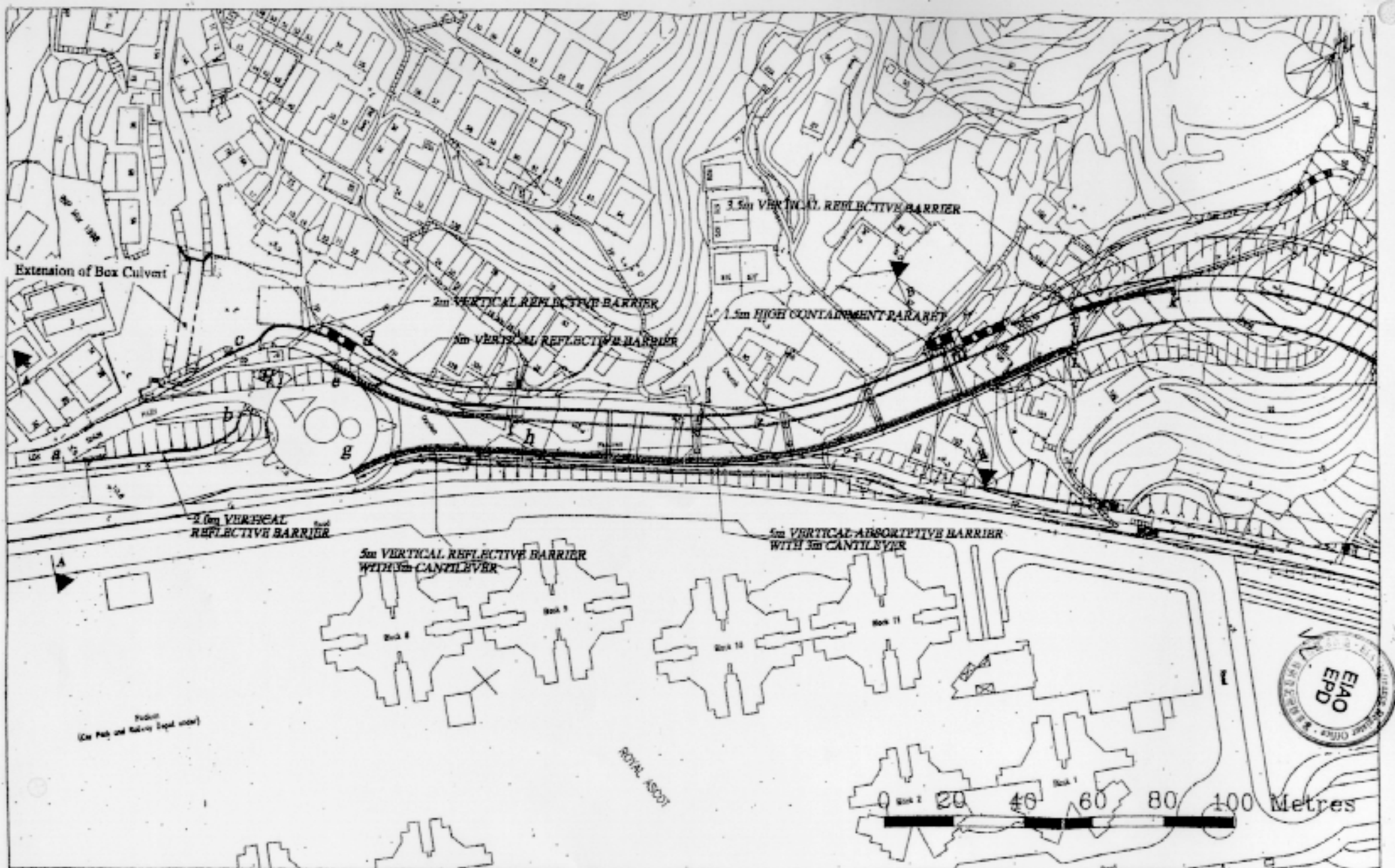
Title Road D15 Linking Lok Shun Path and Tai Po Road Figure 2 - Locations of Proposed Noise Barriers (Reproduced from Figure 2.5 of the Environmental Review attached to the Environmental Permit Application No. AEP-092/2001)
