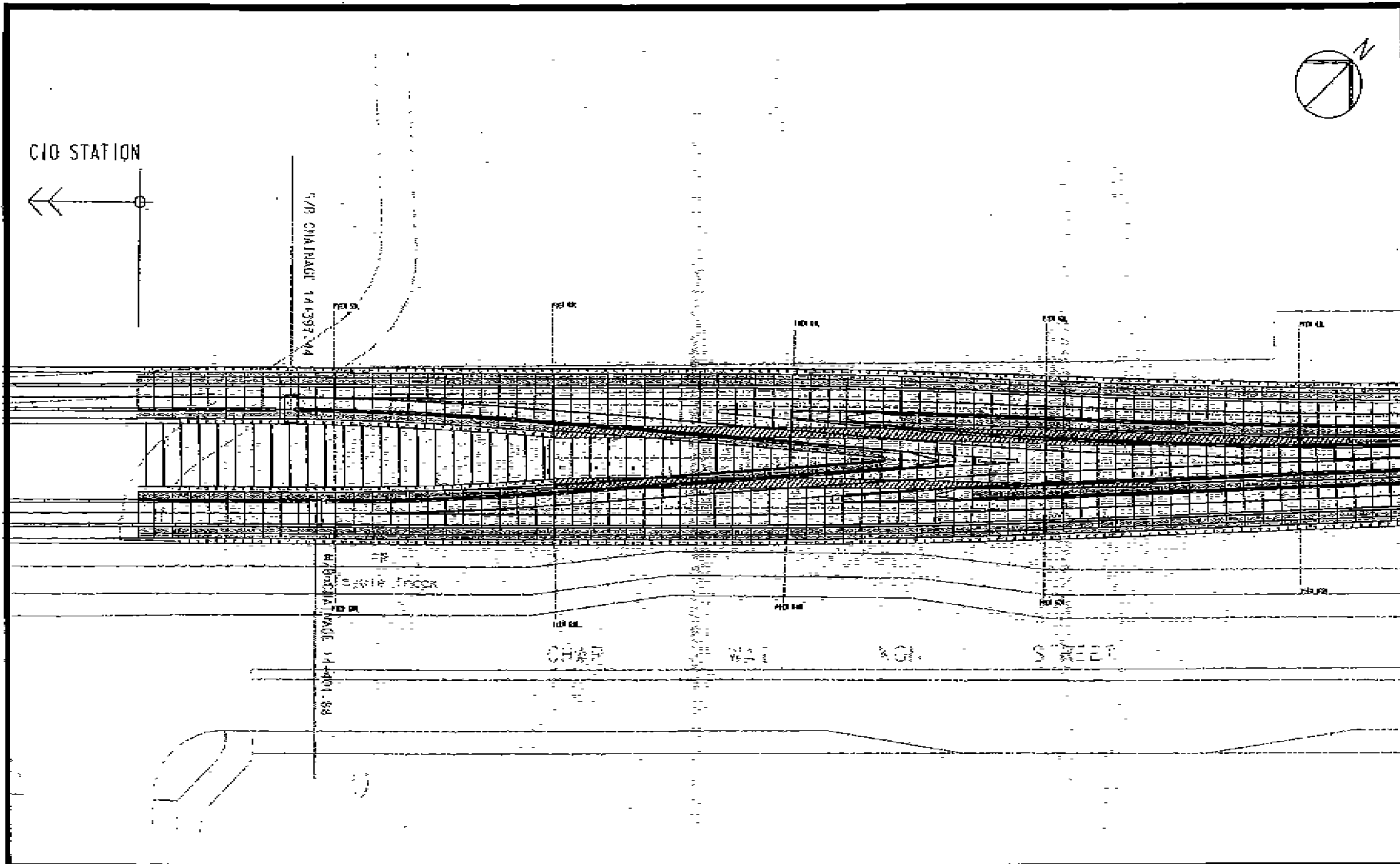
Figure 11 Point machine locations between City One Station and Shek Mun Station (Extracted from the Application VEP-085/2003)
