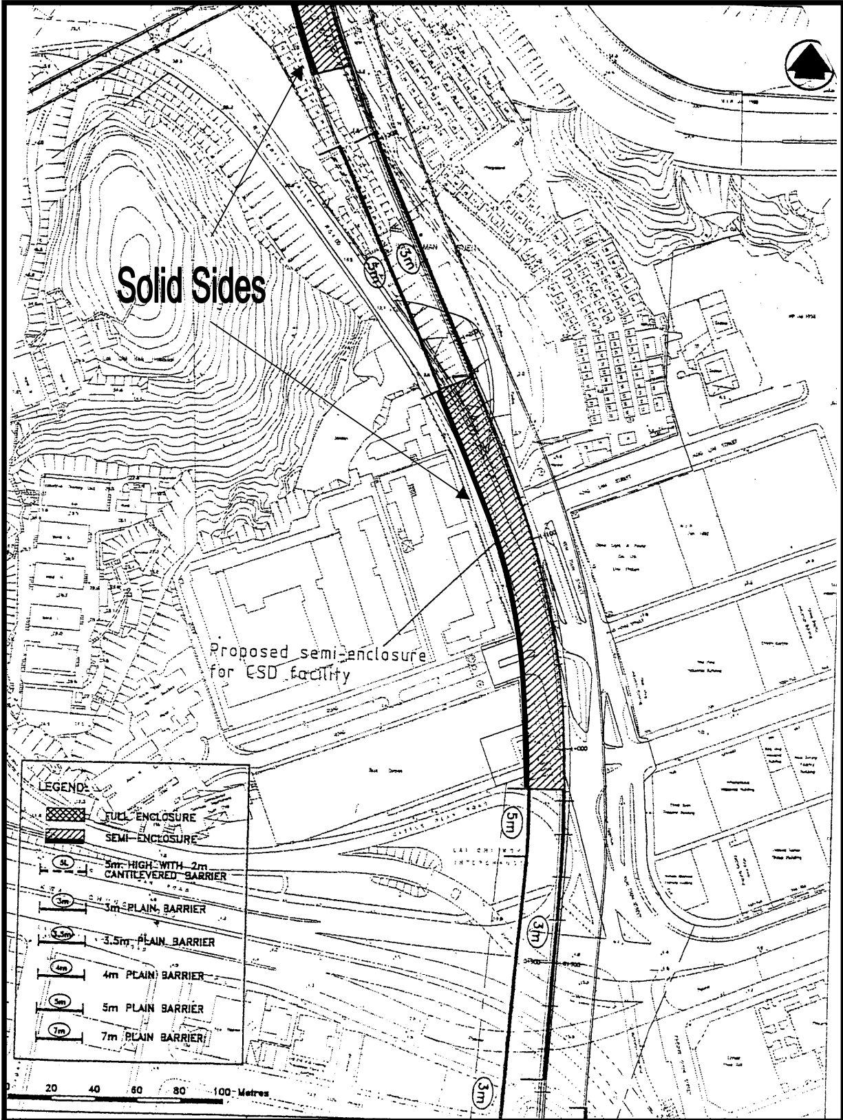
Figure 3 Noise Barriers and Enclosures (Extracted from the Application AEP-103/2001)
