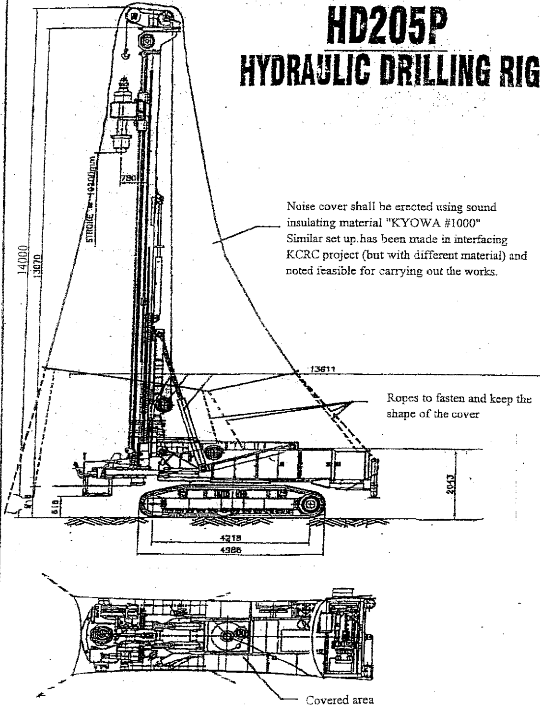
Figure 2(f) Placement of Noise Insulating Material on Piling System and Drilling Rig Extracted from MTRC's Contractor (Kumagai Gumi Co., Ltd) Submission for VEP Application No. VEP-072/2002
