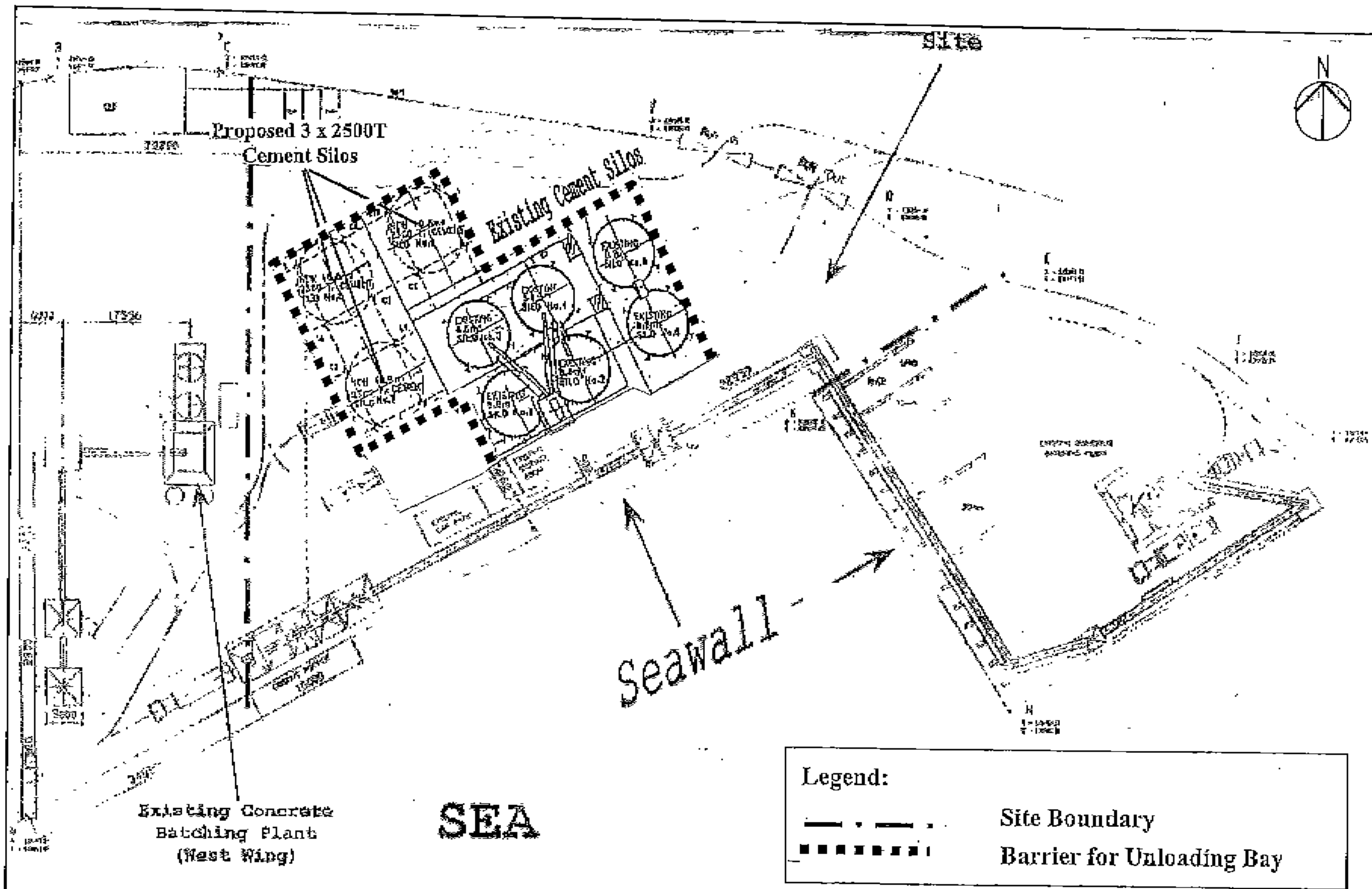
Figure 3 Noise Barriers at the Cement Silos (Extracted from Application VEP-103/2003)
