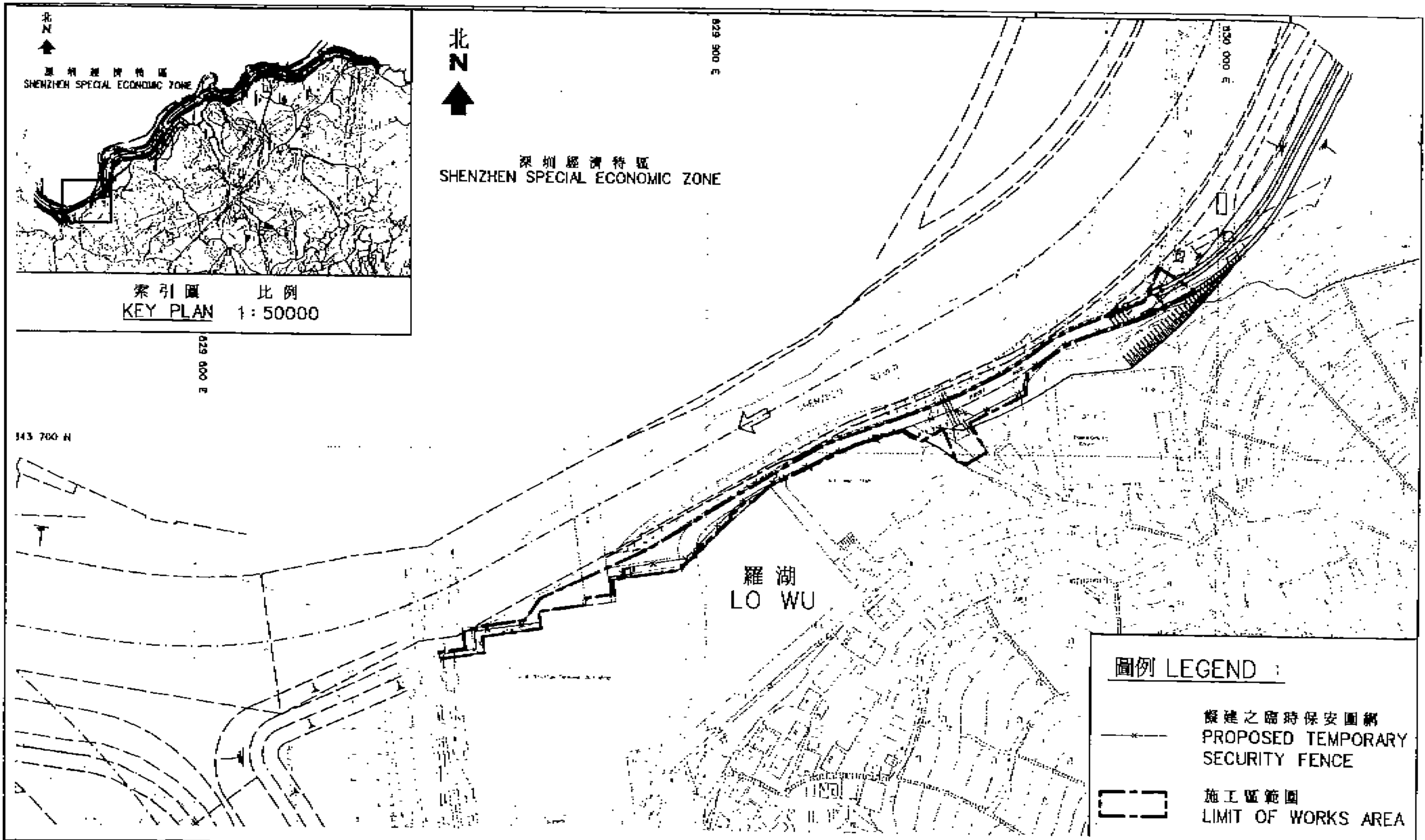
圖 2 治理深圳河第三期工程 — 羅湖臨時保安圍網 Figure 2 Shenzhen River Regulation Project Stage III — Temporary Security Fence at Lo Wu
