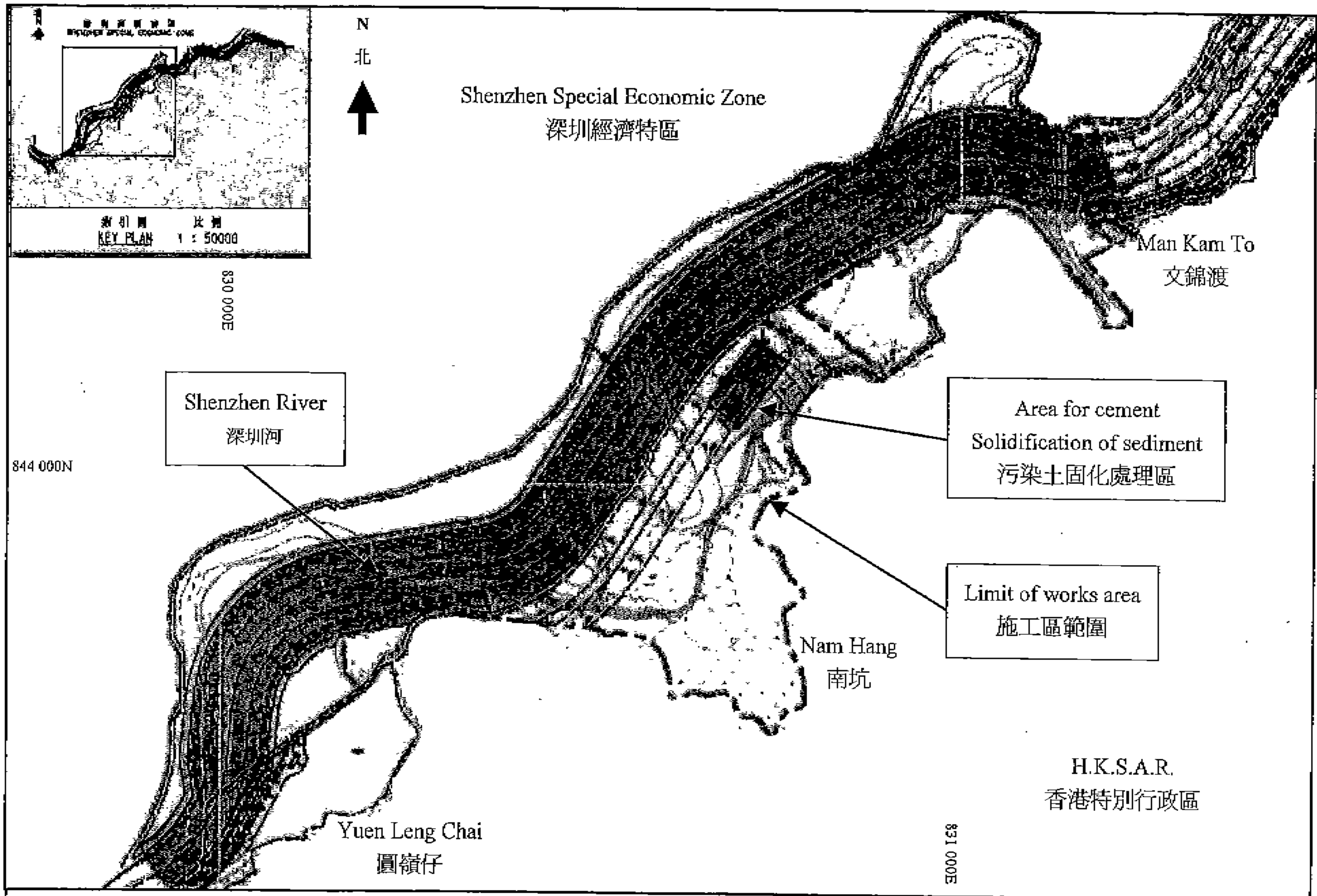
圖 4 治理深圳河第三期工程 - 污染土固化處理及固化物料填築佈置圖 Figure 4 Shenzhen River Regulation Project Stage III — Section of Shenzhen River for sediments solidification and location of area for solidification
