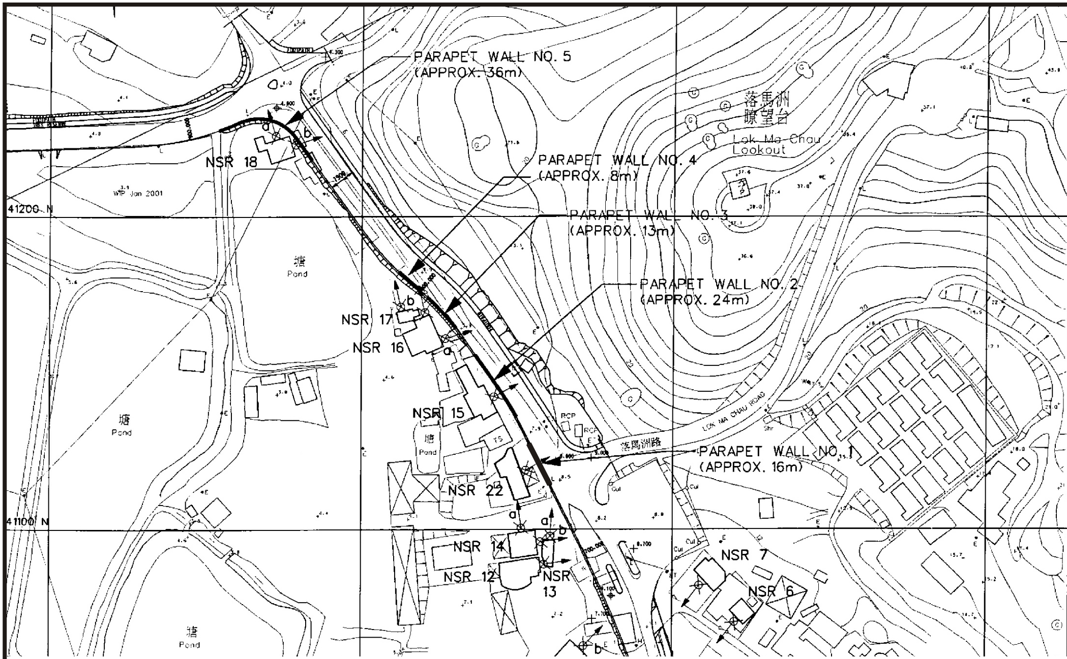
Figure 13 - Location of 0.8m high parapet wall along the Lok Ma Chau Road described in Condition 3.36 of the Permit
