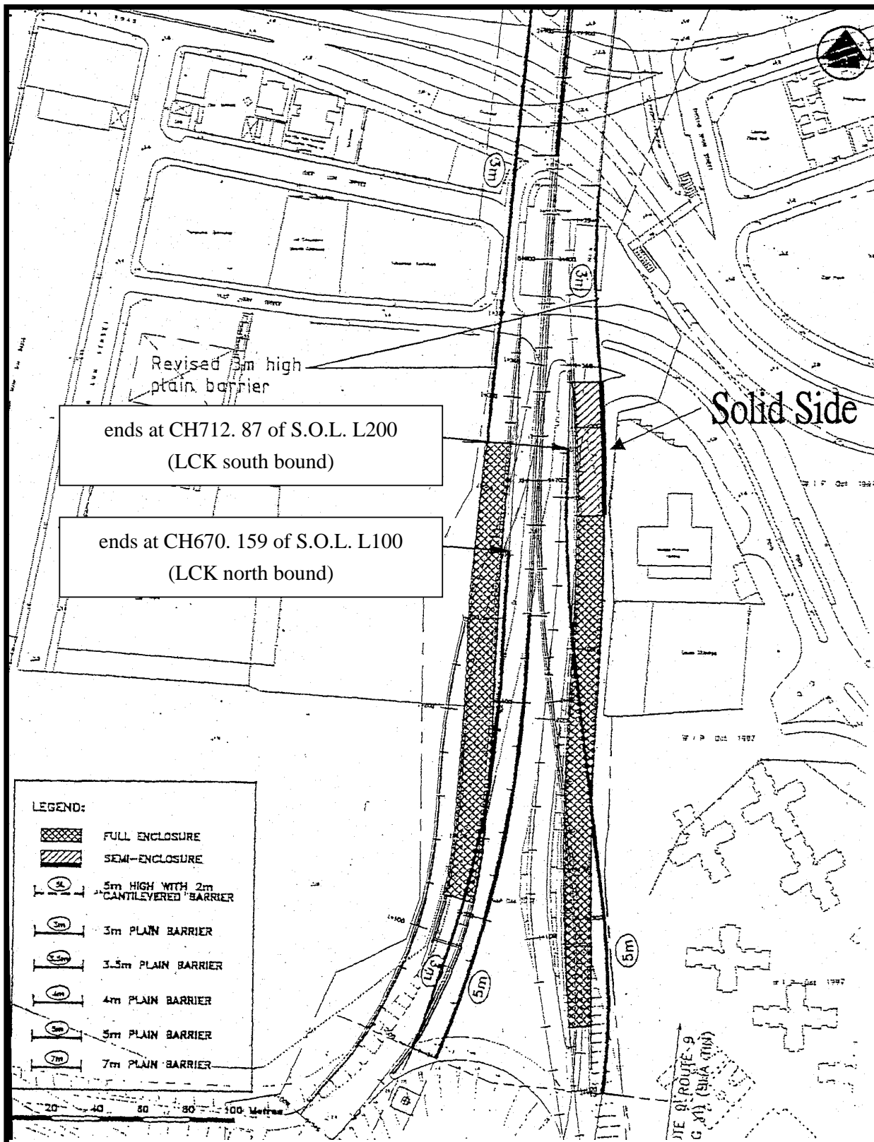
Figure 2 Noise Barriers and Enclosures (Extracted from the Application VEP-094/2003)
