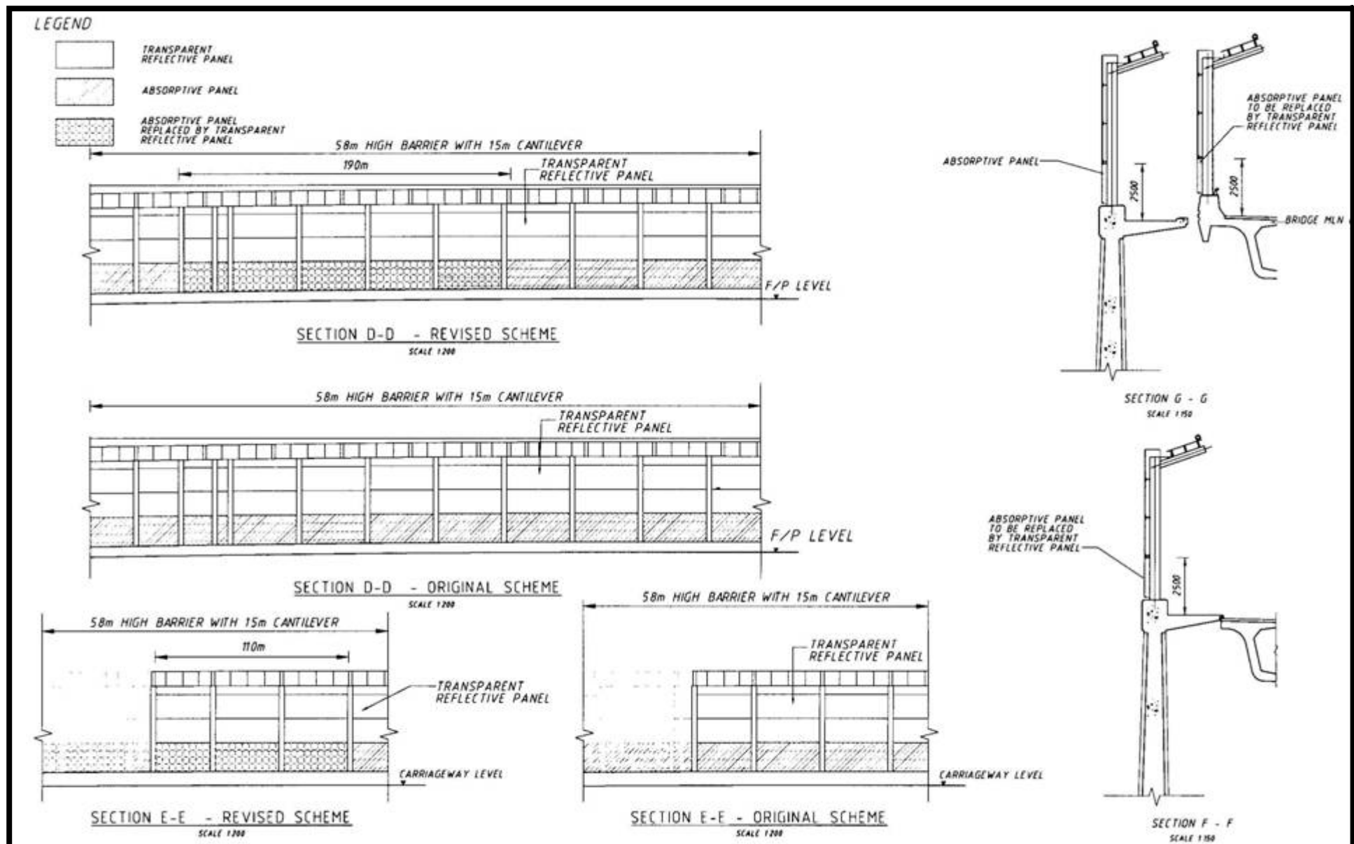
Sha Tin New Town – Stage II, Road T3 and Associated Roadworks Figure 13 – Extent of noise barrier segment no. 31 where absorptive panels as originally provided to a height of 2.5m above the road level are replaced by transparent reflective panels (Extracted from the Application VEP-169/2005)
