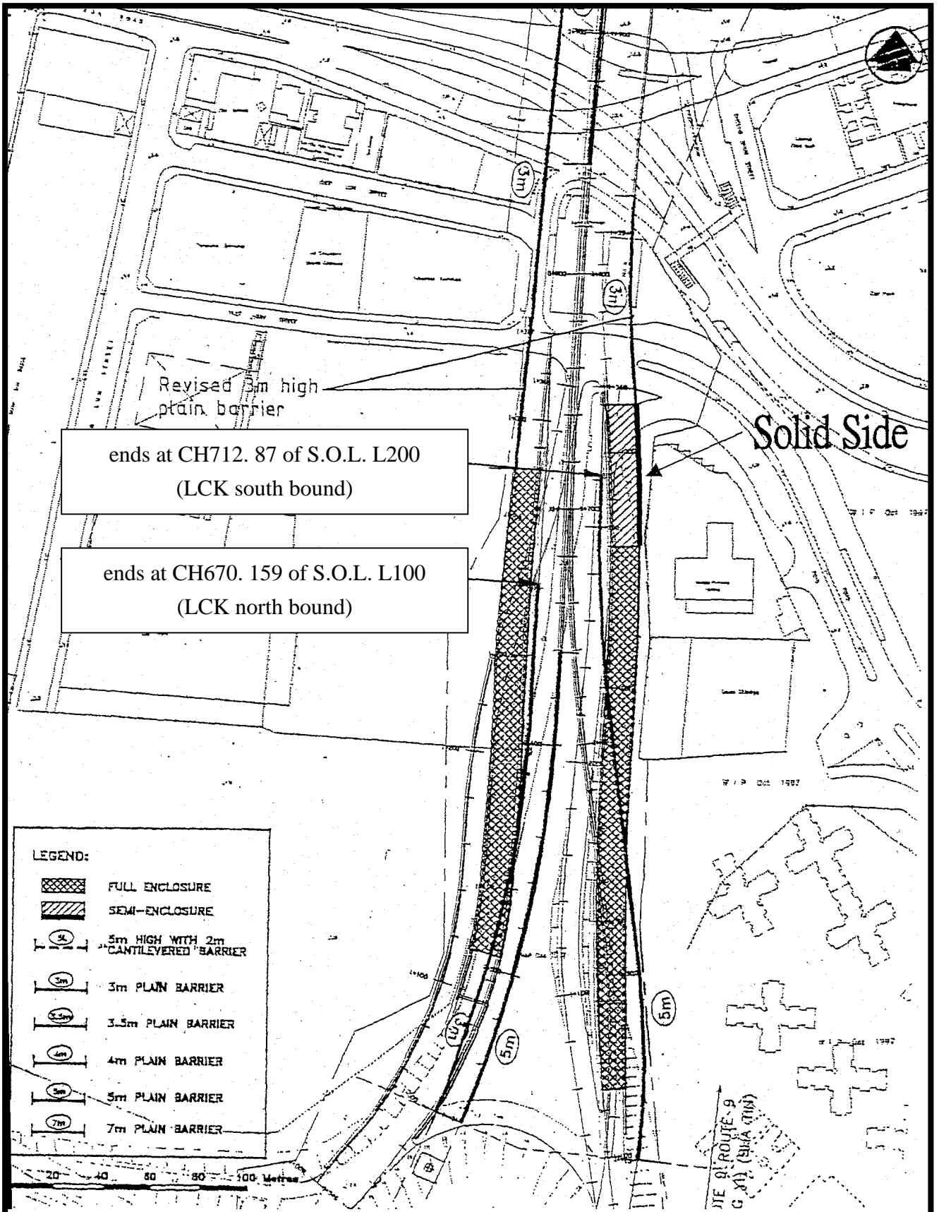
Figure 2 Noise Barriers and Enclosures (Extracted from the Application VEP-180/2005)
