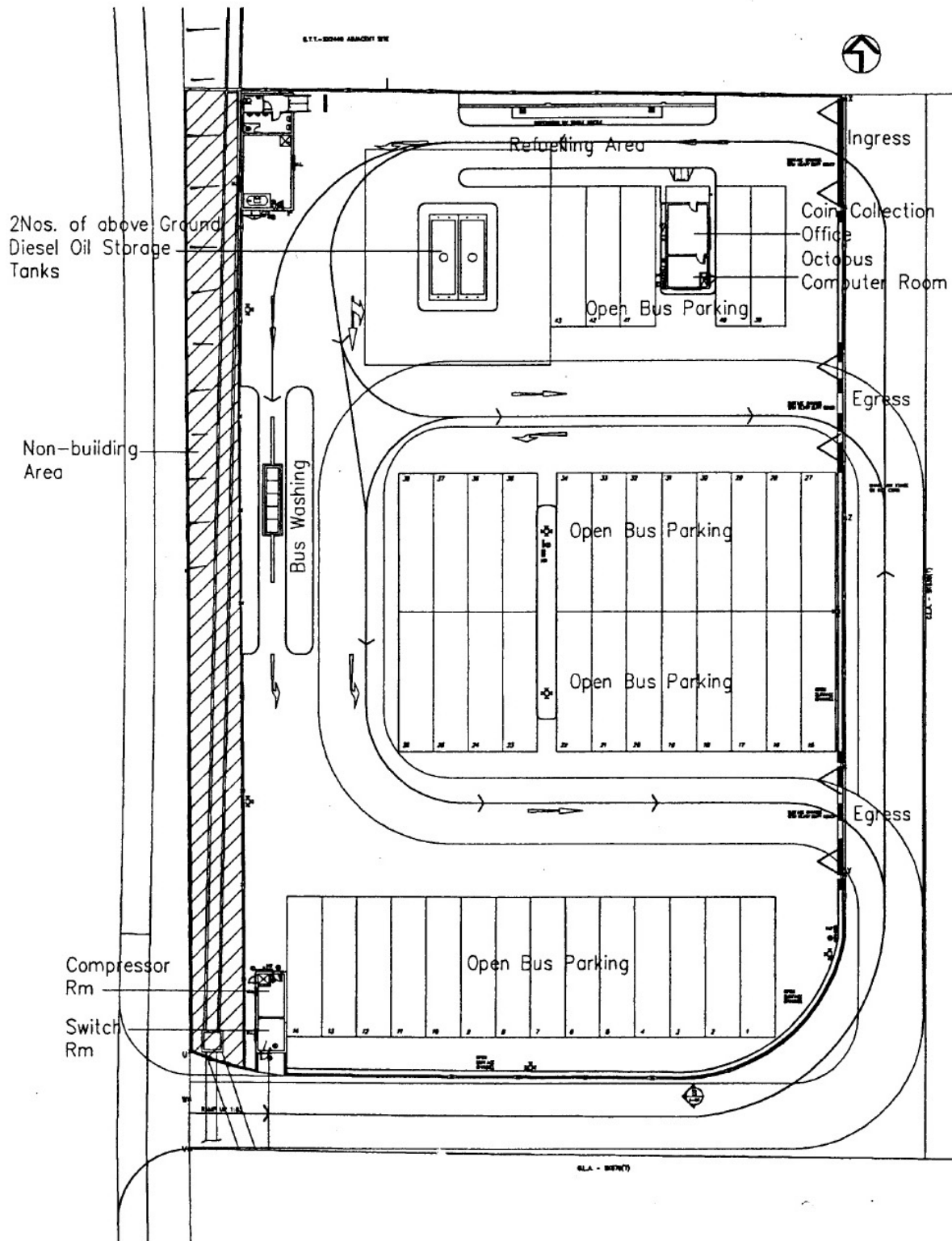
Figure 2 : Layout Plan of the Proposed Temporary Bus Depot at Tseung Kwan O, Area 85
