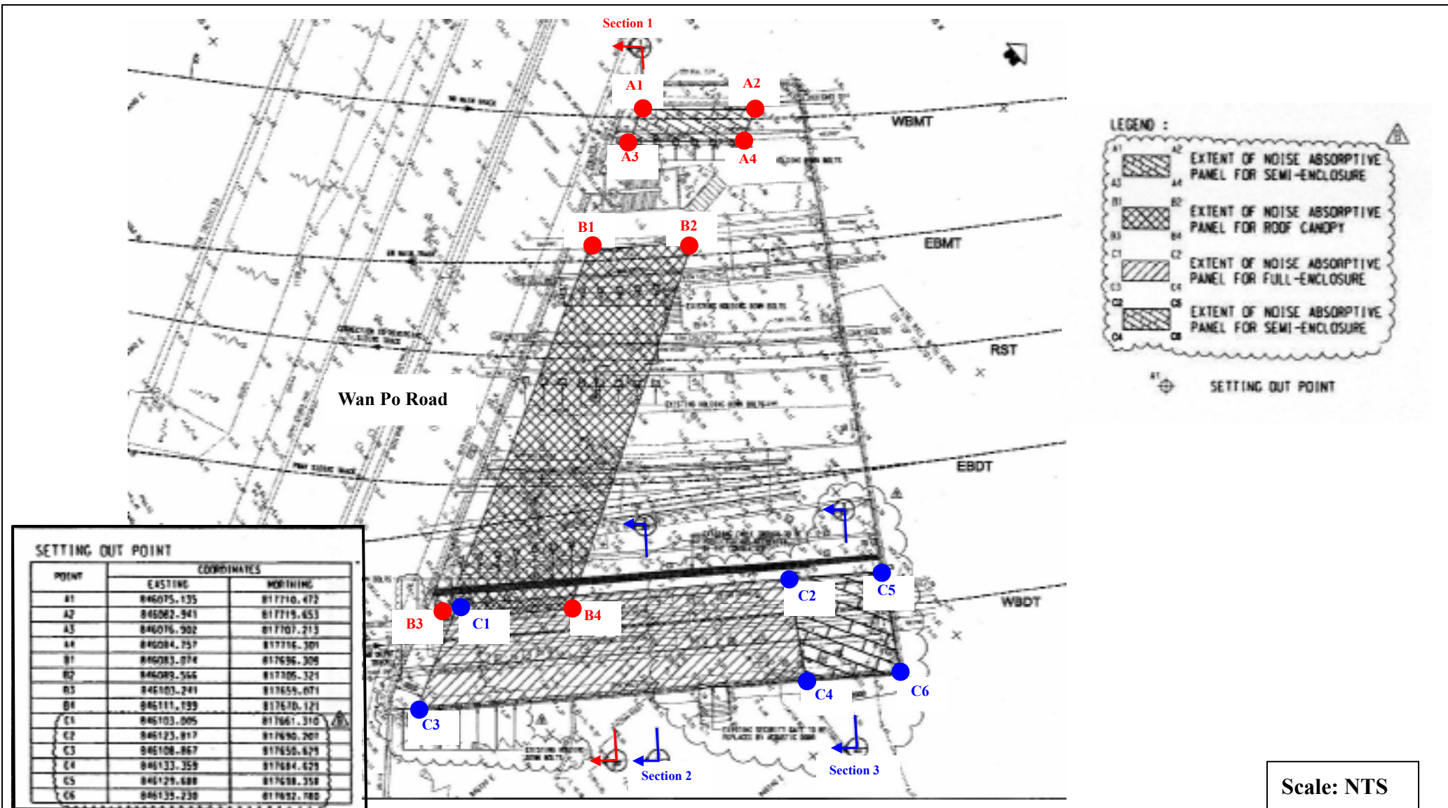
Figure F – Proposed Location and Length of the Noise Barriers along the Main Track, Reverse Siding Track and Depot Track
