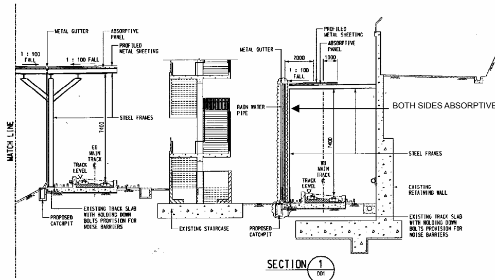
Figure G – Proposed design of the Noise Barriers (Typical Section 1)
