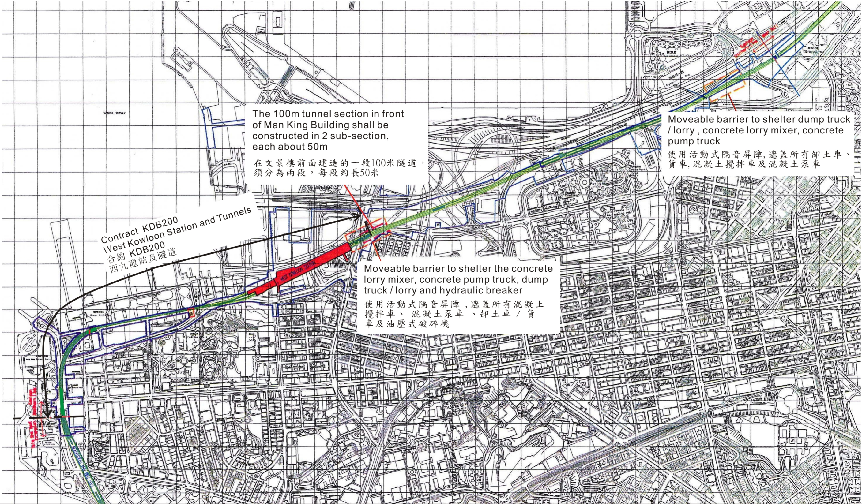
Figure 3 : Specific Mitigation Measures for Particular Powered Mechanical Equipments at Worksites in front of Man King Building and Olympic City Phase III 圖 3 : 為文景樓及奧海城三期前面的工地內某些機動設備，採取特定的緩解措施
