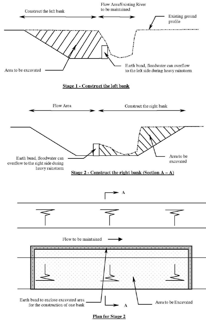
Figure 2: Dry Working Method for Excavation in River (Ref. Drg. No. 5.2 of the EIA Report)
