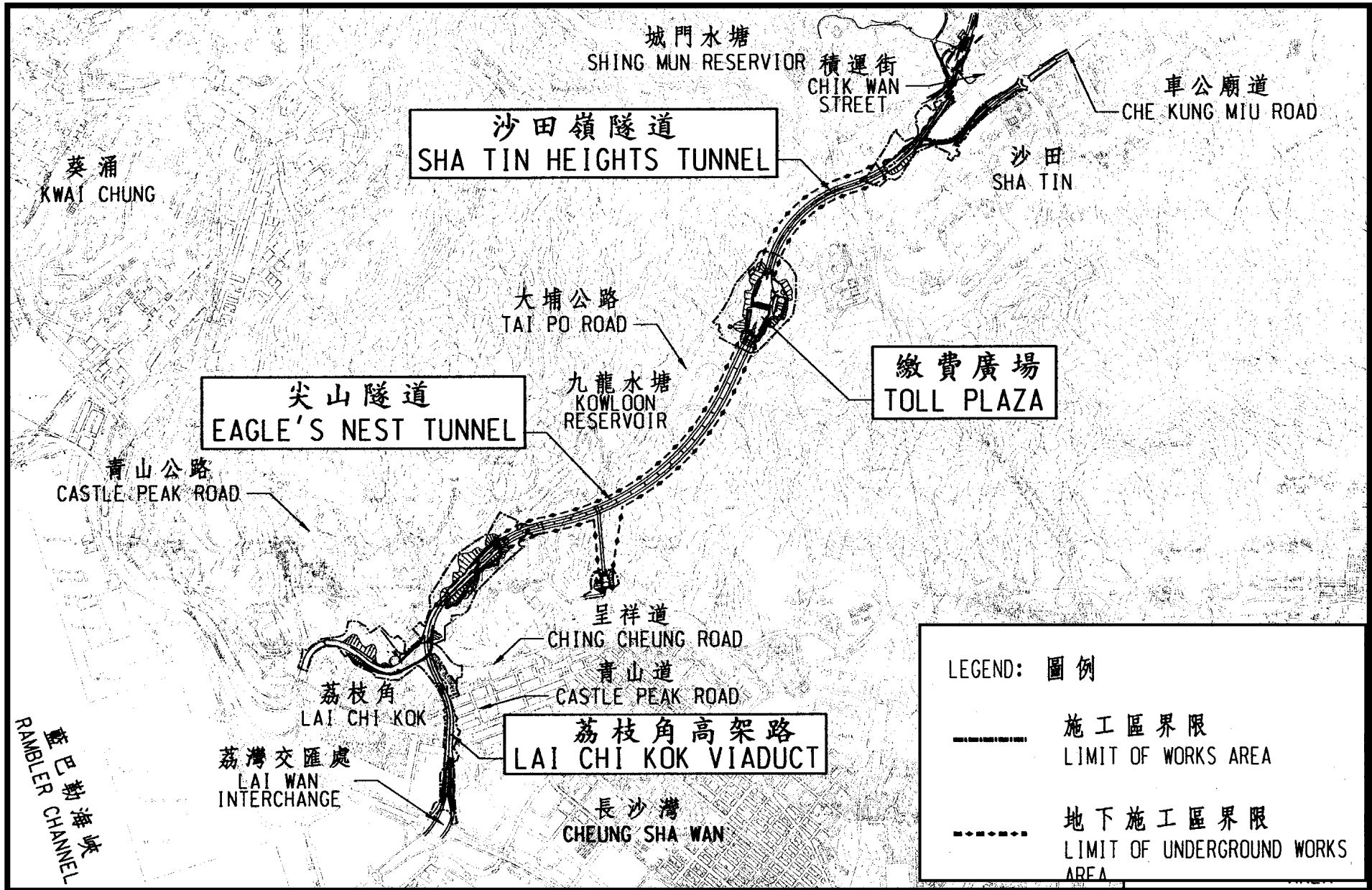
Figure 1 Location Plan for Route 9 between Cheung Sha Wan and Sha Tin (Extracted from the Application VEP-180/2005)
