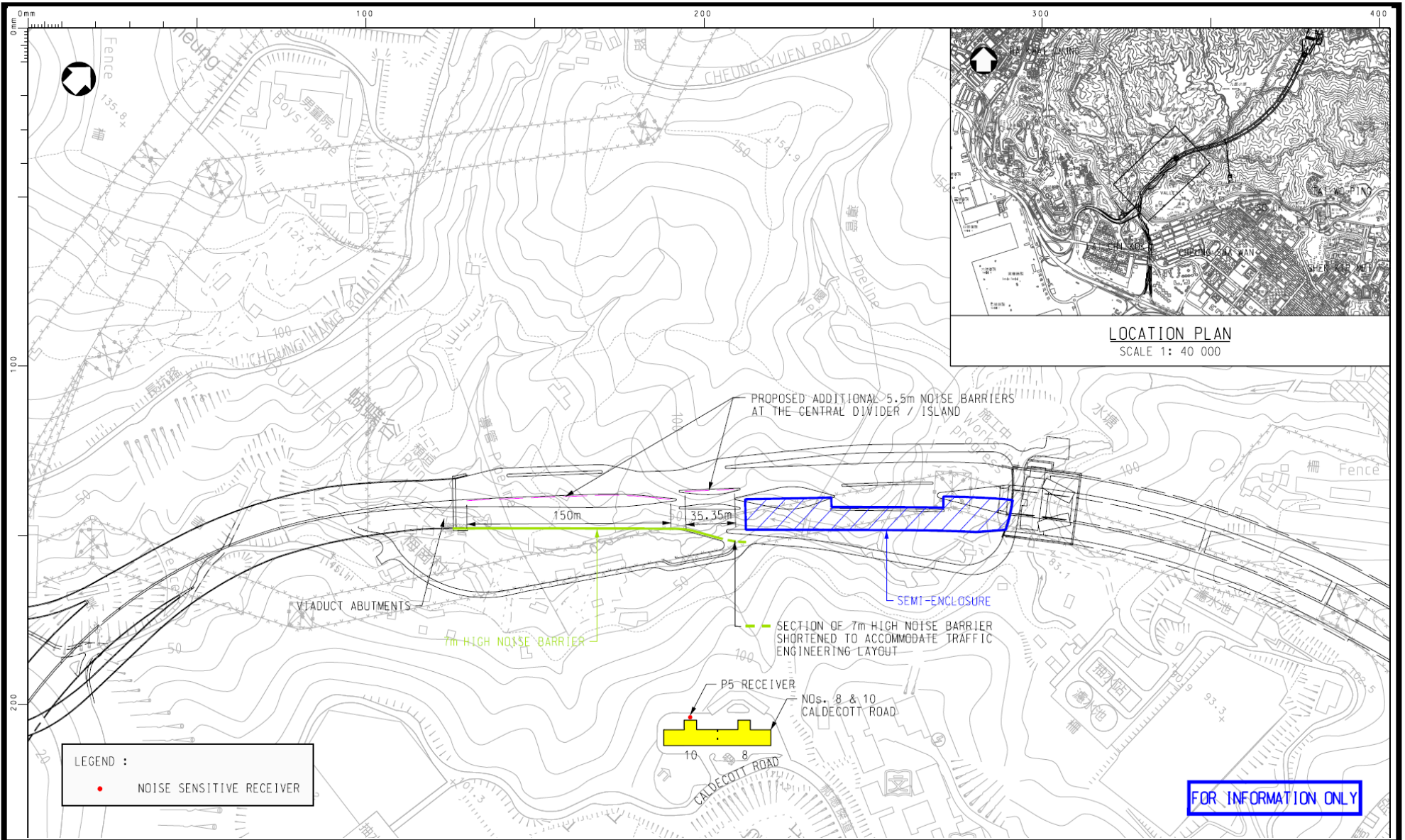
Figure 6 Variation to Noise Barriers (Extracted from the Application VEP-256/2008)
