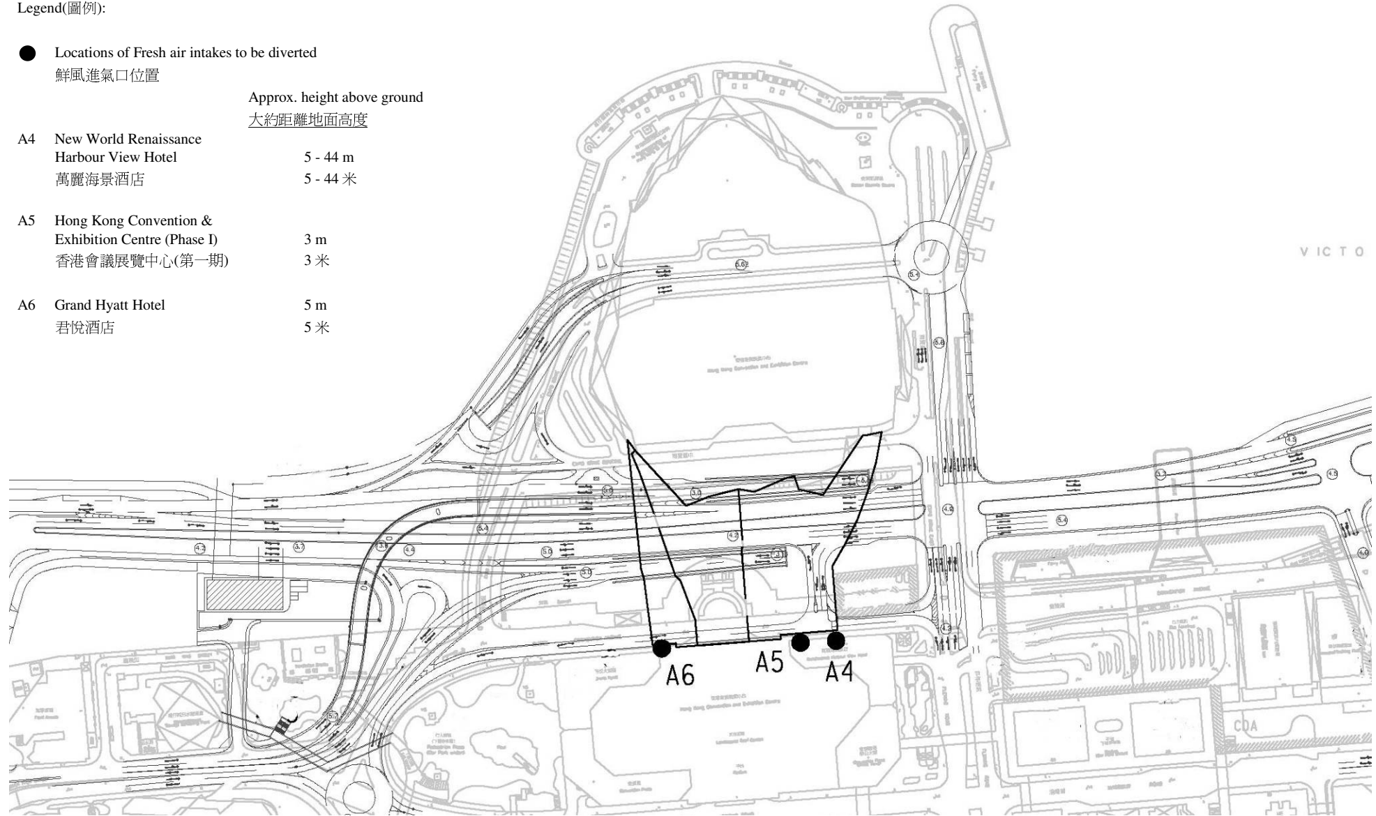
Figure 4: Locations of Fresh Air Intakes to be Diverted 圖 4: 需要改動的鮮風進氣口位置
