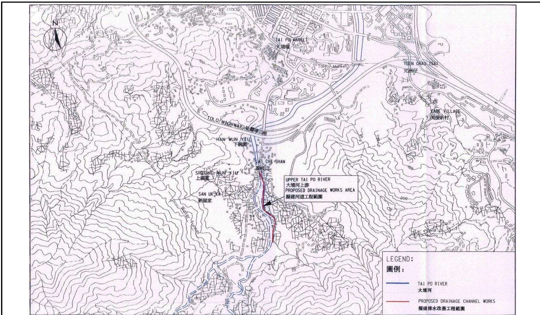
Figure 1: Drainage Improvement Works in Upper Tai Po River – Location Plan
