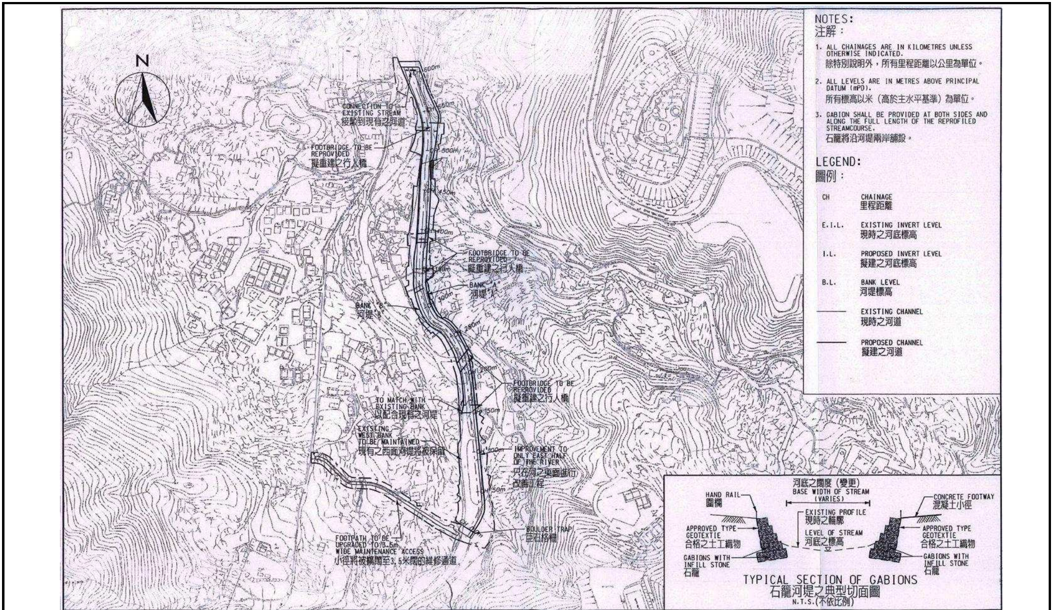
Figure 2: Drainage Improvement Works in Upper Tai Po River – General Layout Plan
