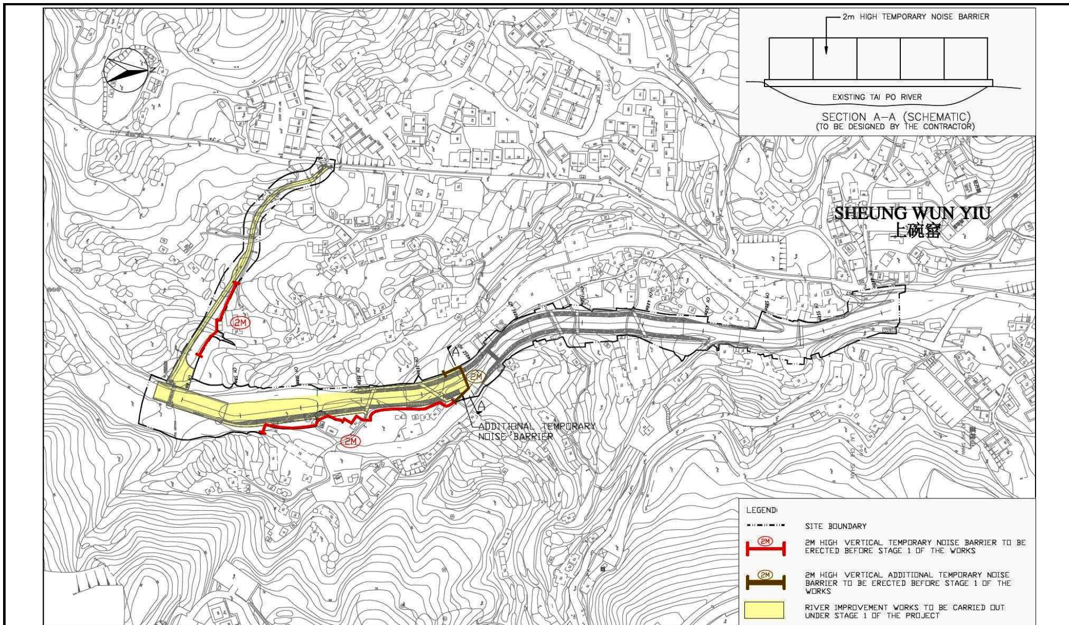
Figure 3: Drainage Improvement Works in Upper Tai Po River
