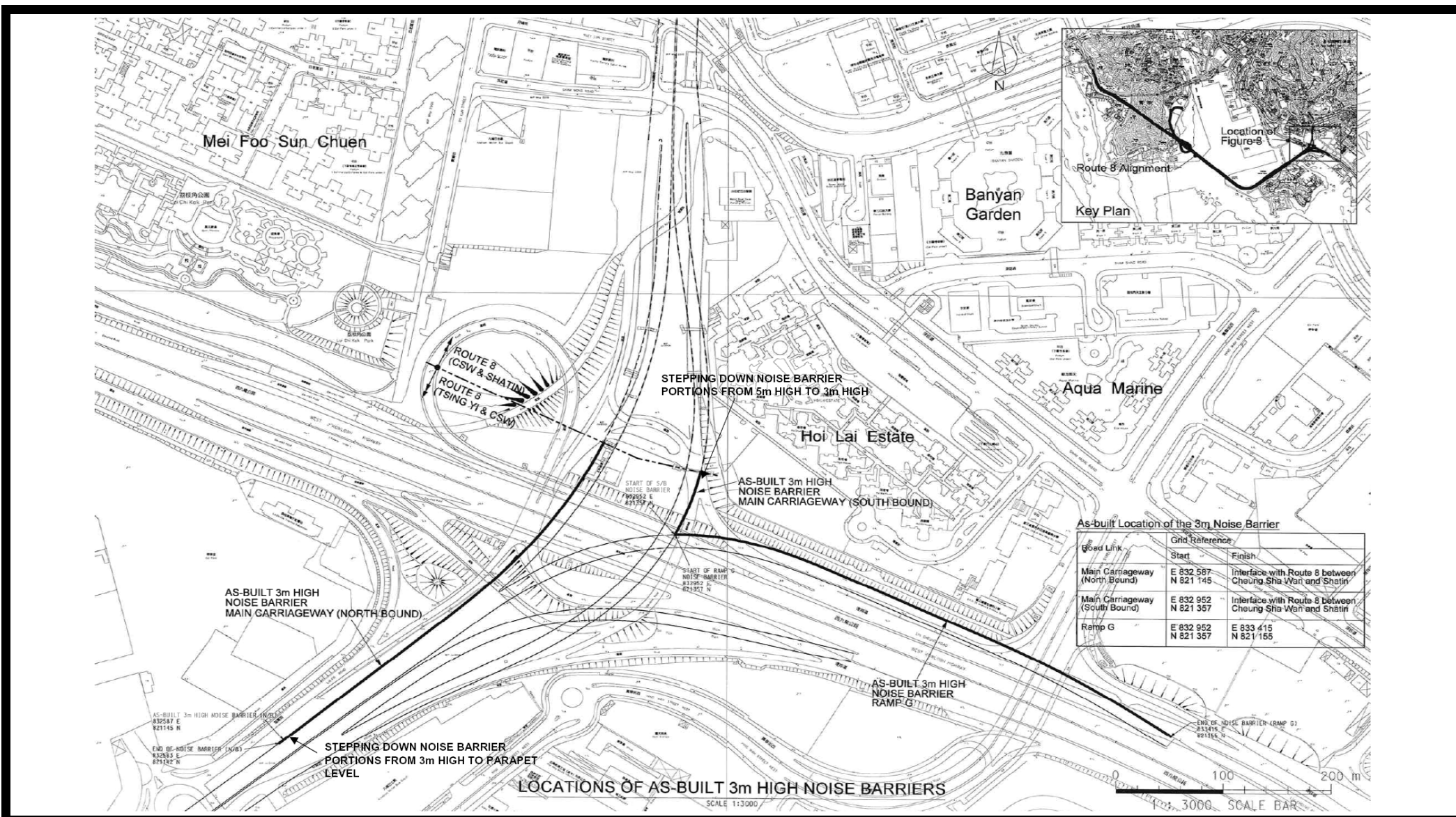
Figure 3: Locations of As-Built 3m High Noise Barriers (Scale : NTS)
