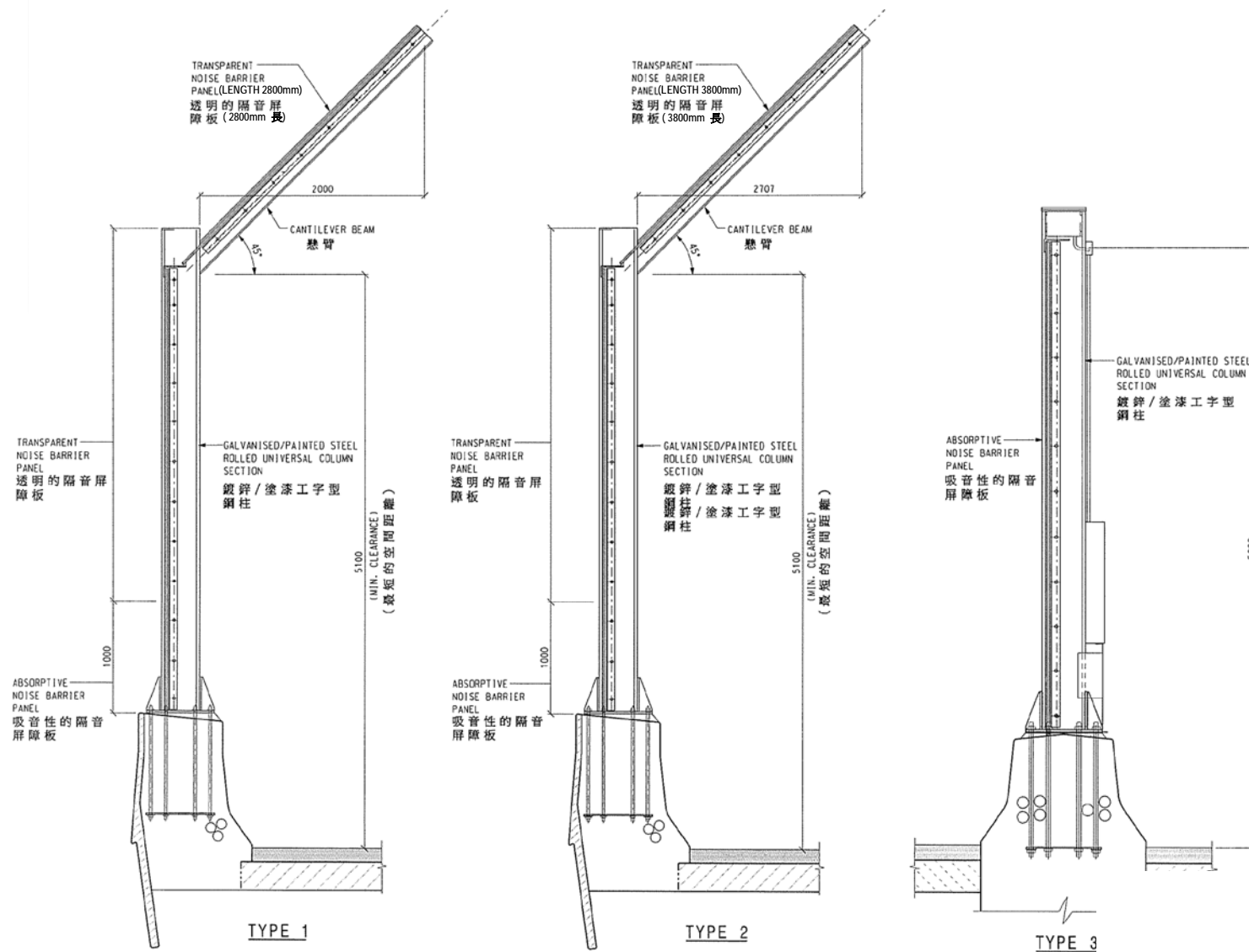
Figure 4: Typical Section of Noise Barriers on Sliproads Linking to Container Terminal 9
