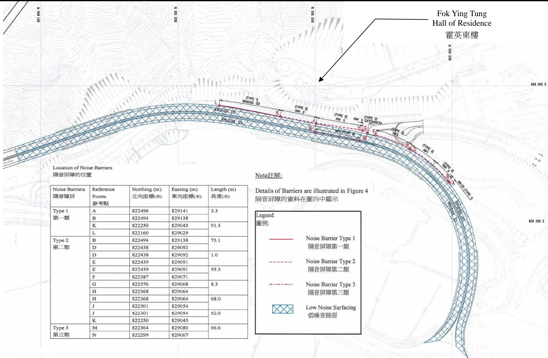
Figure 5: Locations of Barrier on Sliproads linking to Container Terminal 9 (Scale : NTS)
