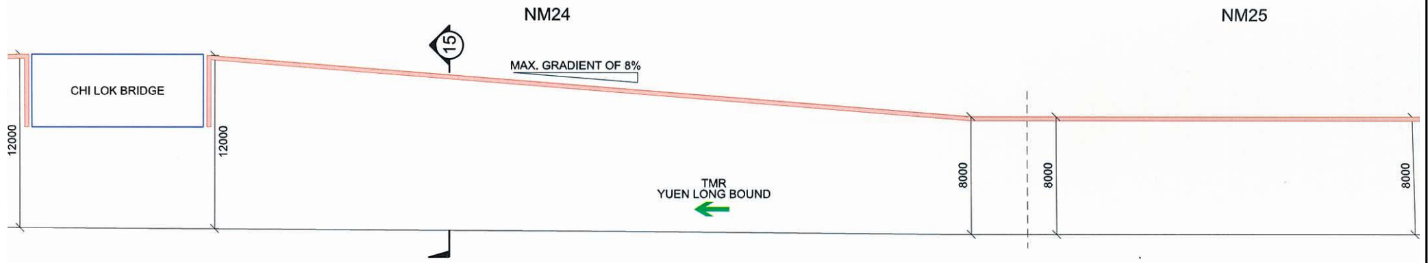
LONGITUDINAL SECTION ALONG TMR YUEN LONG BOUND BETWEEN NM24 AND NM25 (N.T.S.)
