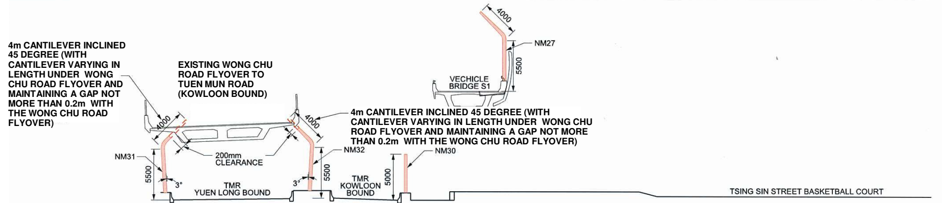
SECTION 18-18 BARRIER NM31 and BARRIER NM32 (N.T.S.)
