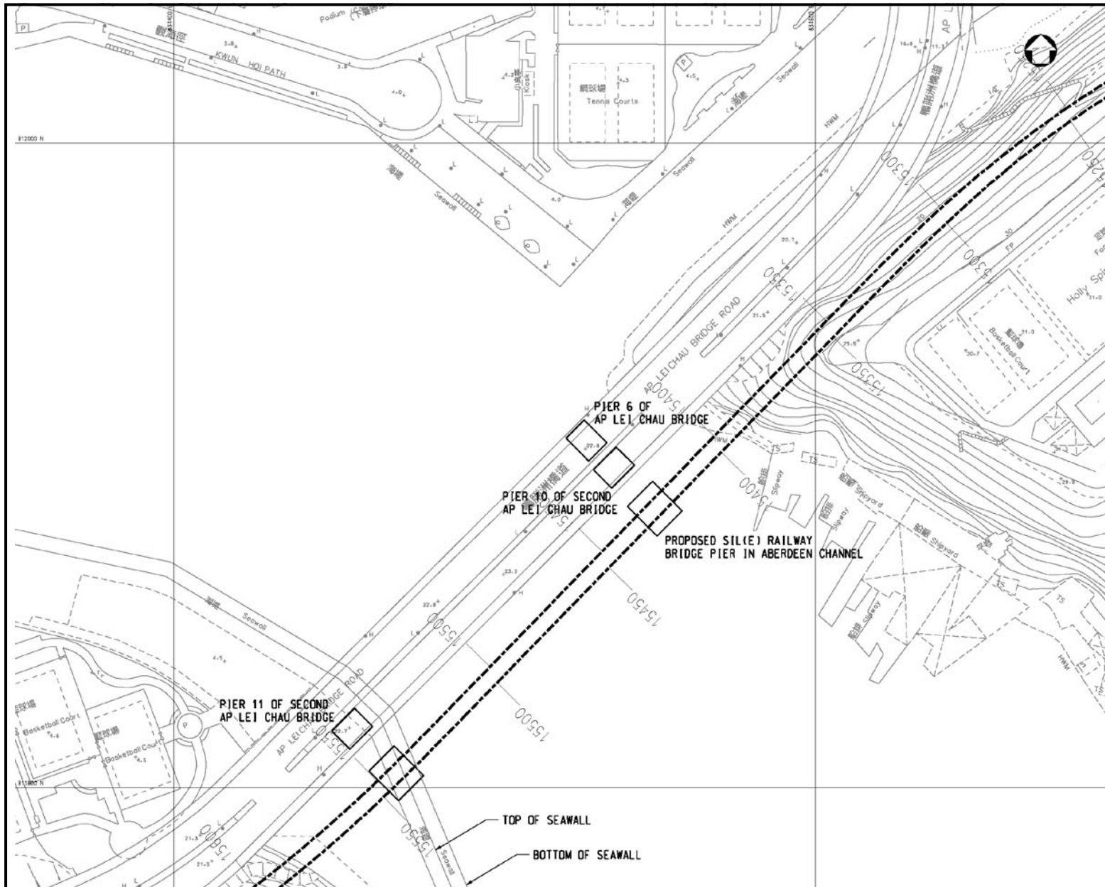
Figure 8: Railway Bridge Pier Foundation
