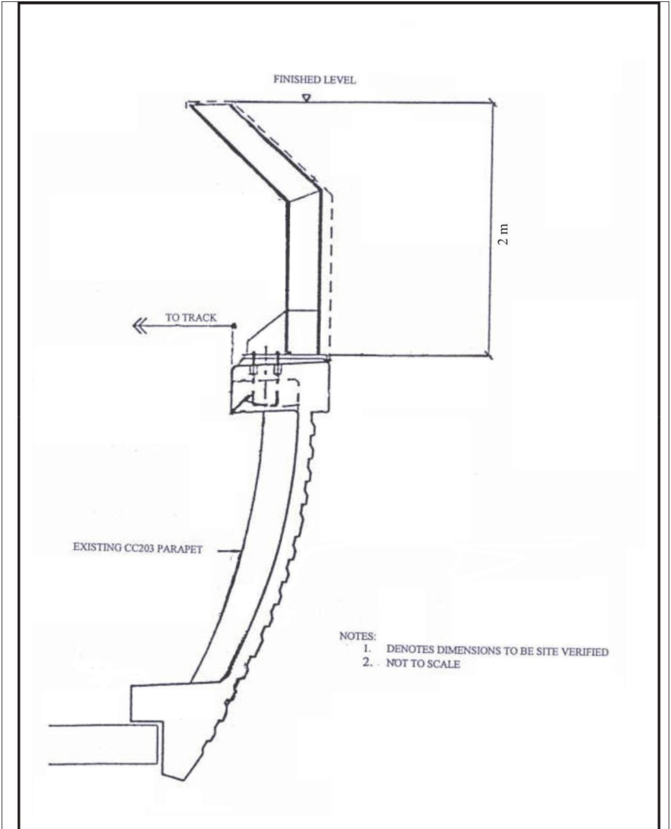
Figure 10 – Cranked Noise Barrier at the Tin Shui Wai Station 圖 十 – 天水圍站的曲軸隔音屏障
