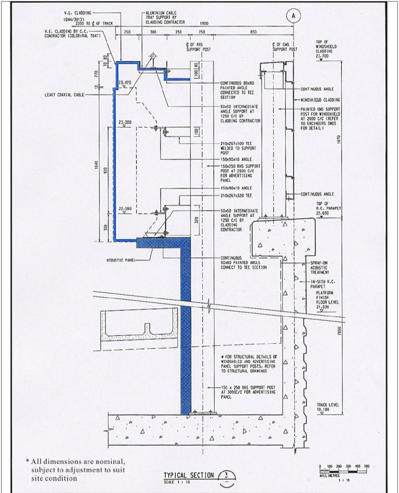
Figure 5 – Trackside Panels and Windshields at the Yuen Long Station [Utrack (track from Kowloon to Tuen Mun)]
