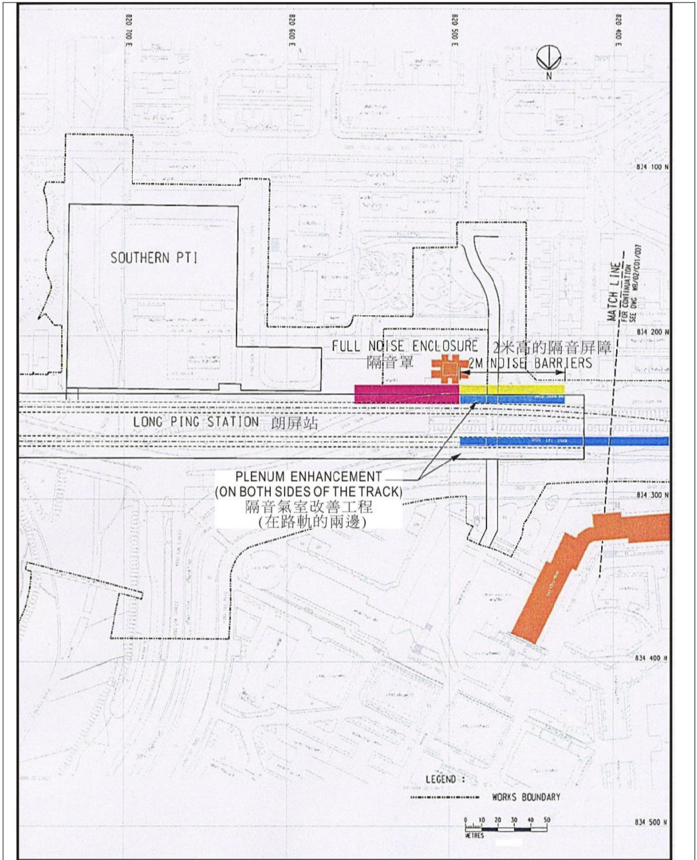
Figure 7 – Tracking Enclosure, 2m Noise Barrier and Plenum Enhancement at the Long Ping Station 圖七 – 朗屏站的路軌隔音罩，2 米高的隔音屏障及隔音氣室的改善工程
