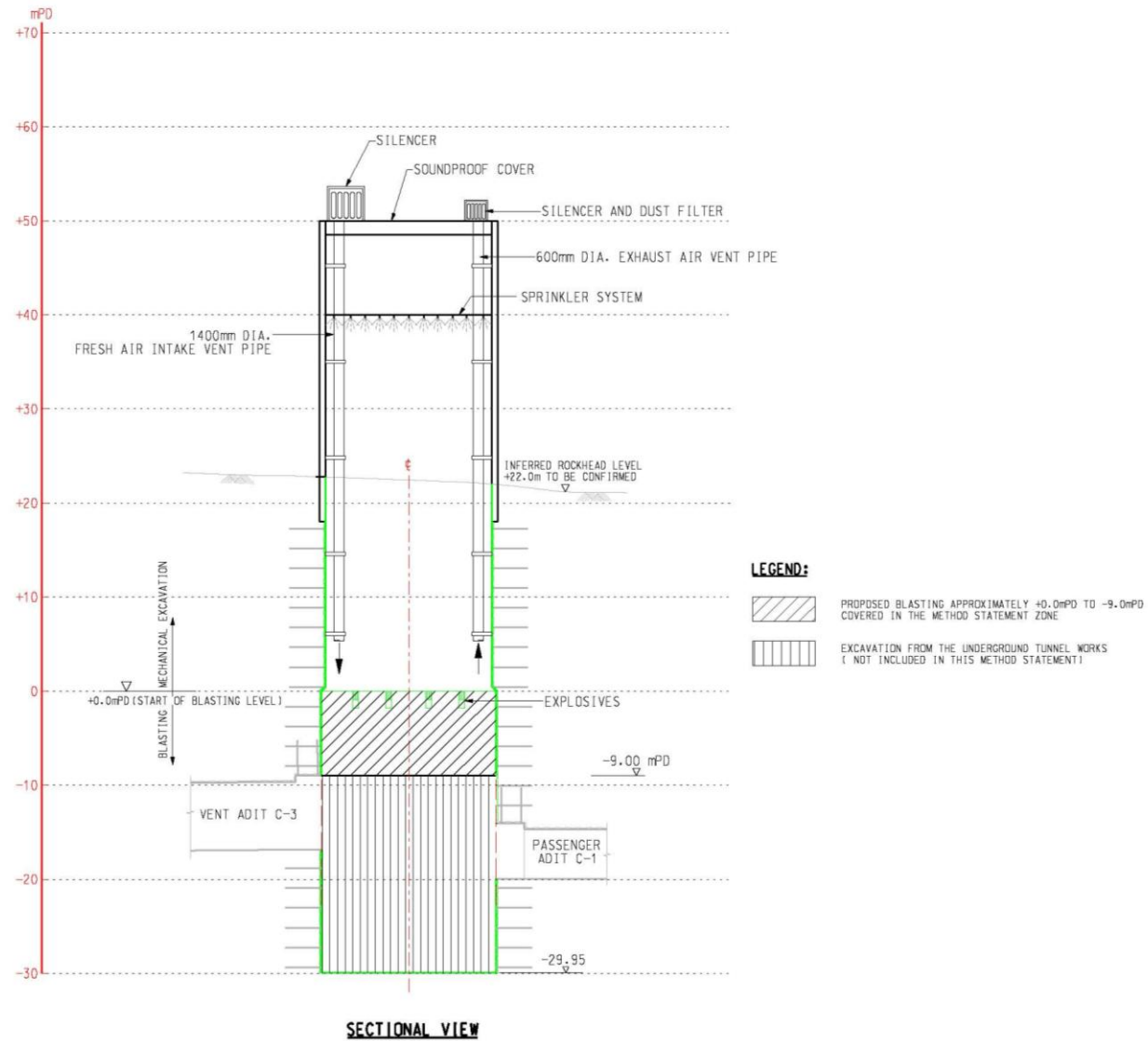
Figure 13: Mitigation Measures for Blasting at Works Area M3 圖 13: 施工區 M3 爆破工程的緩解措施
