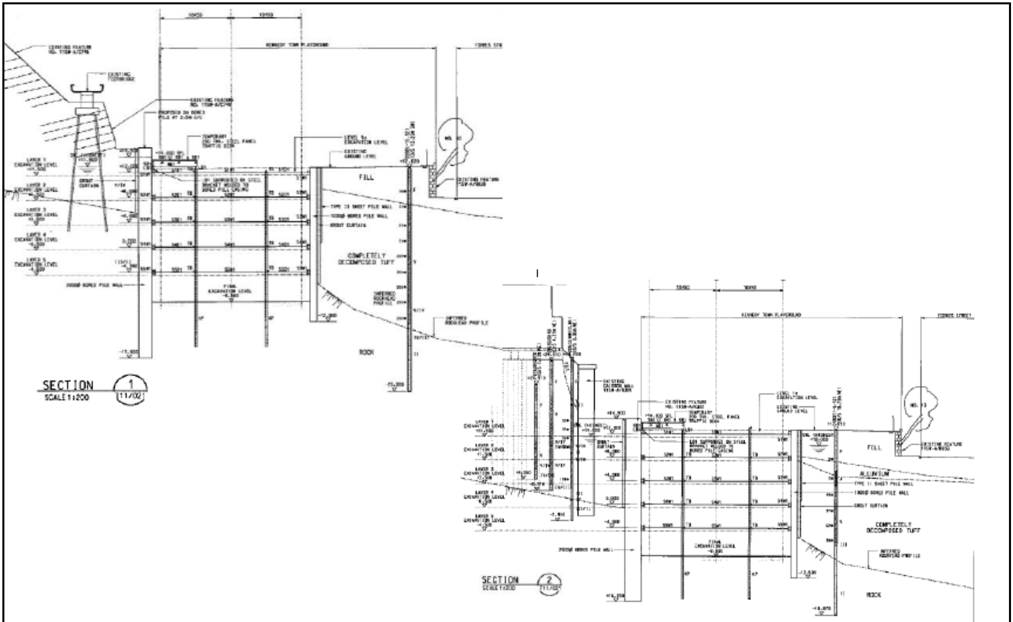
Figure 11: Sections of Decking at Works Area C 圖 11: 施工區內的大概鋪蓋切面圖
