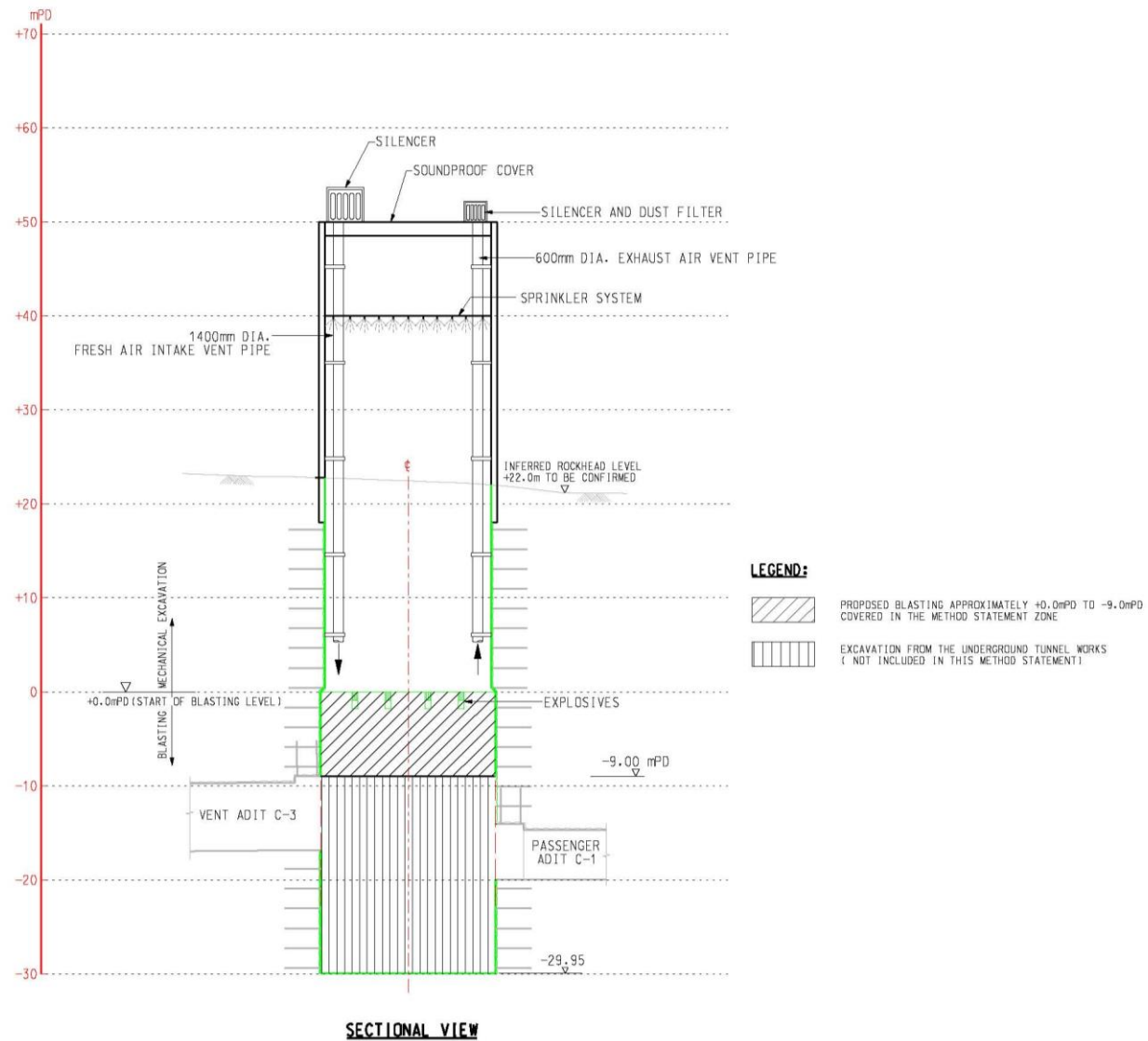
SECTIONAL VIEW
