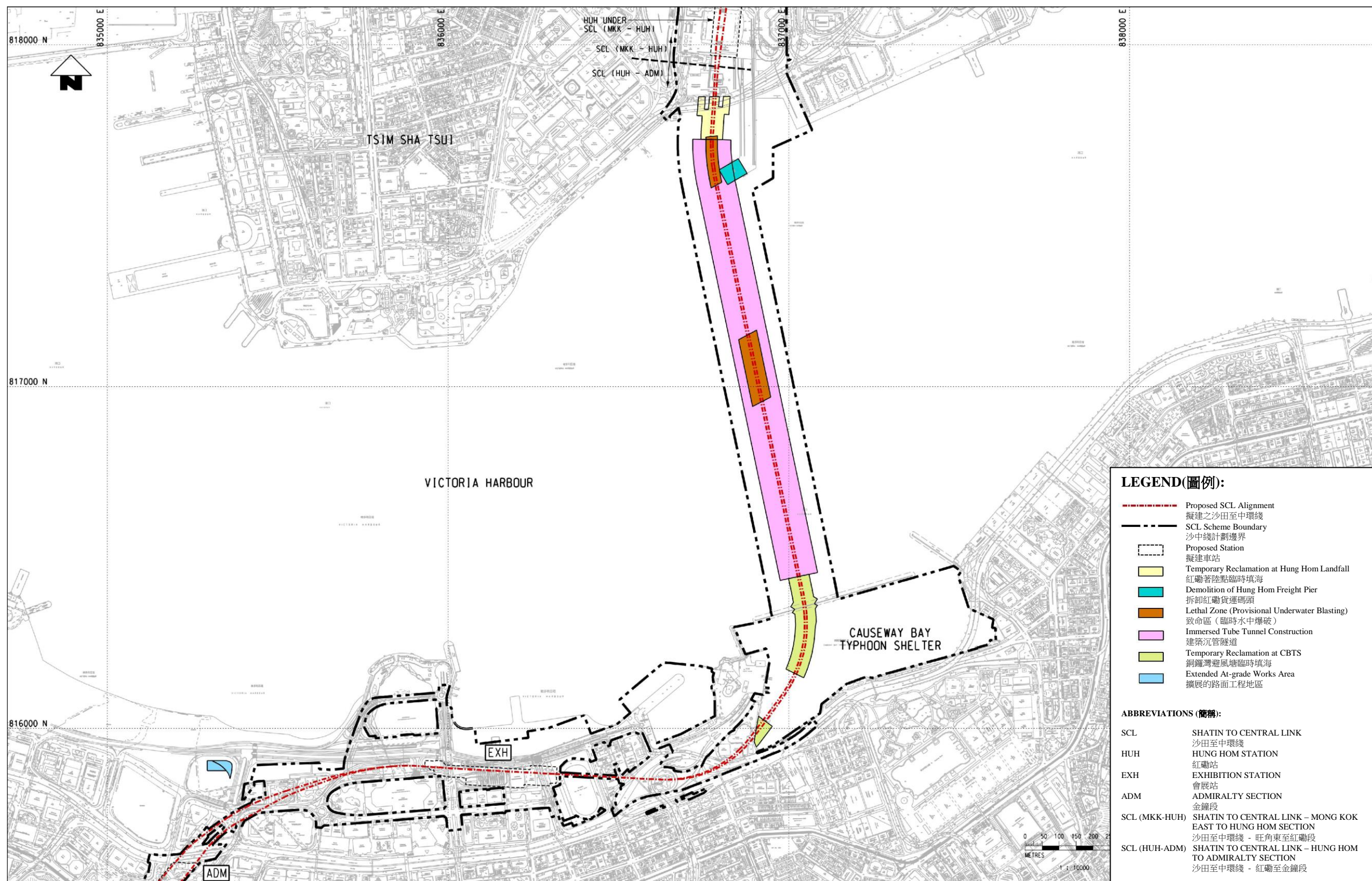
Figure 2: Marine Works for Shatin to Central Link – Hung Hom to Admiralty Section within Victoria Harbour
