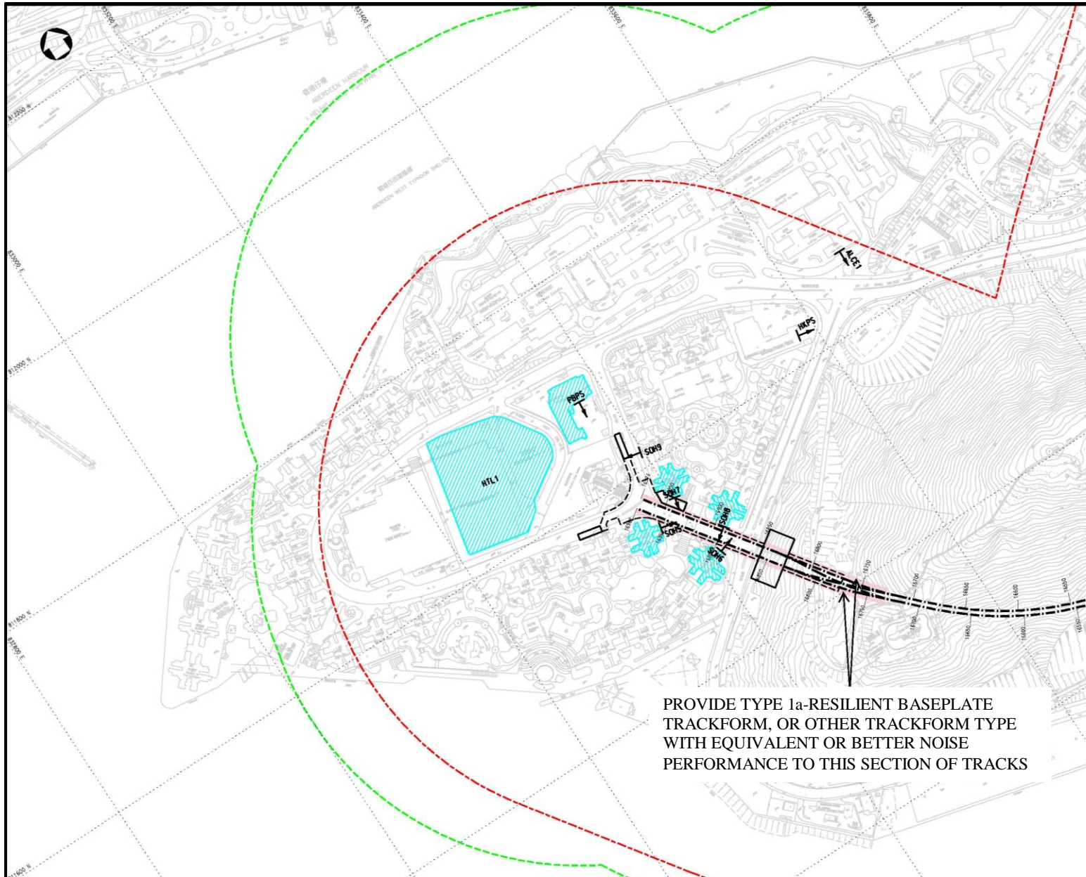
Figure 10: Noise Mitigation Measures for Operational Ground-Borne Noise Near South Horizons Station
