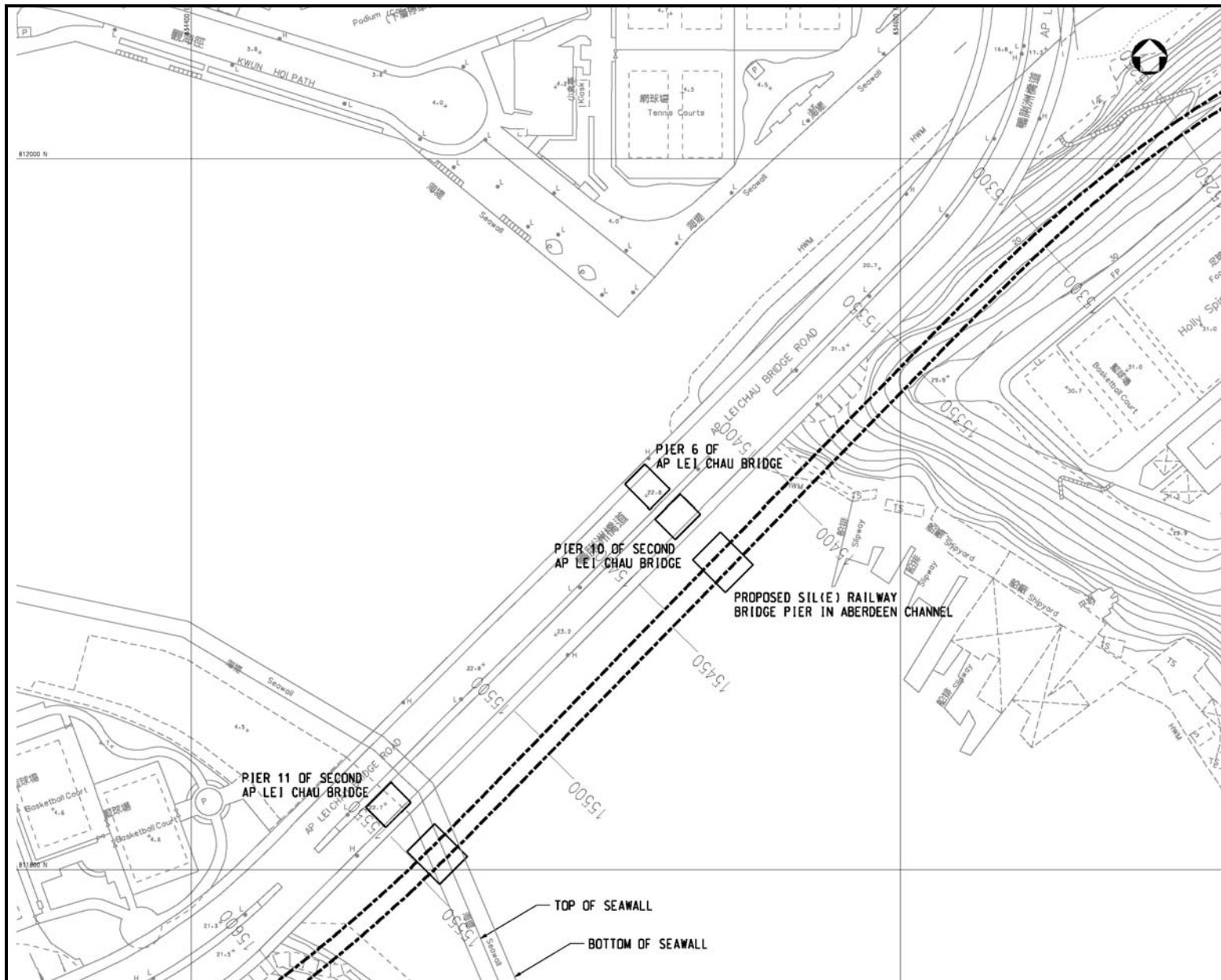
Figure 8: Railway Bridge Pier Foundation 圖 8: 鐵路橋的橋墩地基
