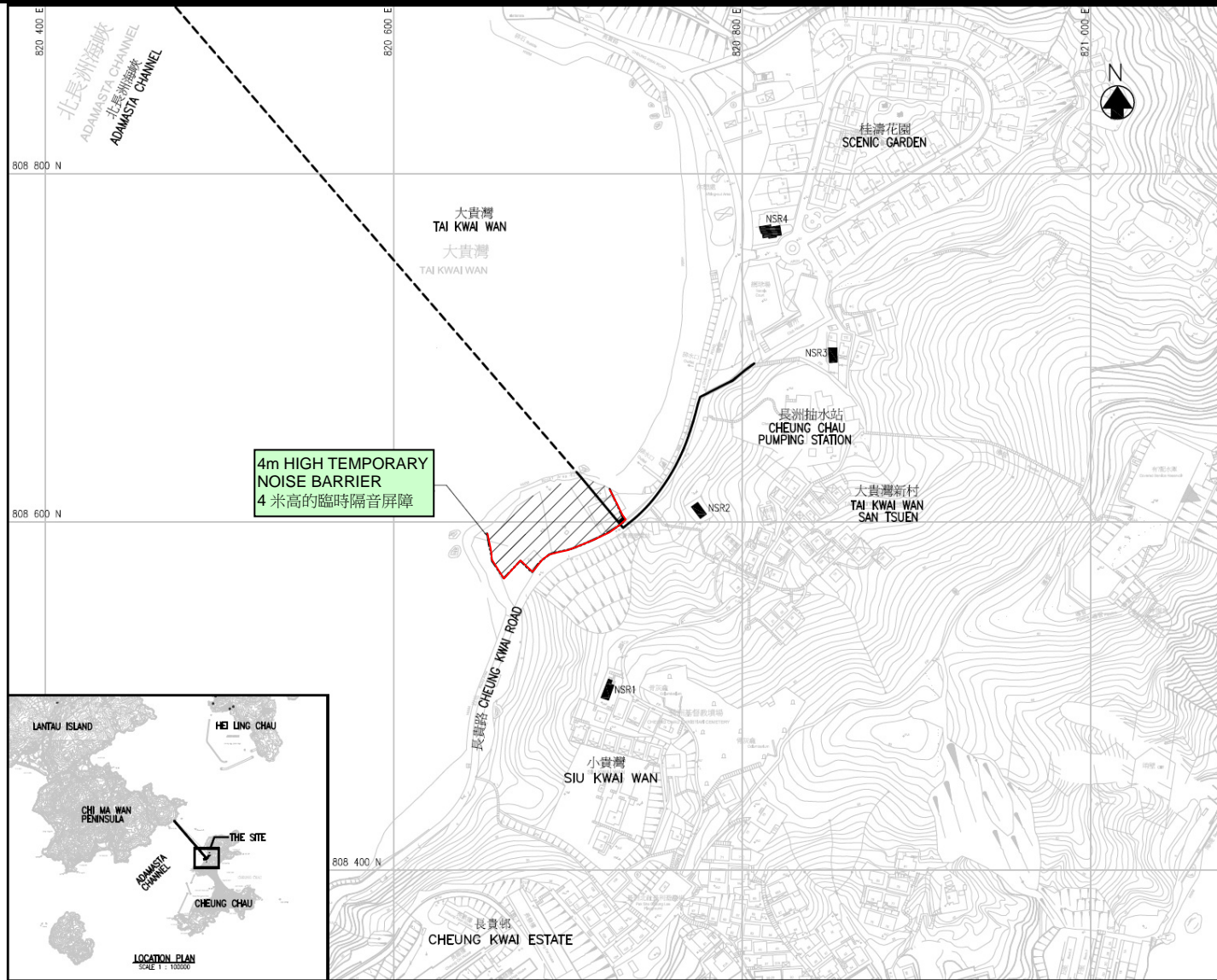
Figure 6: Location of Temporary Noise Barrier
